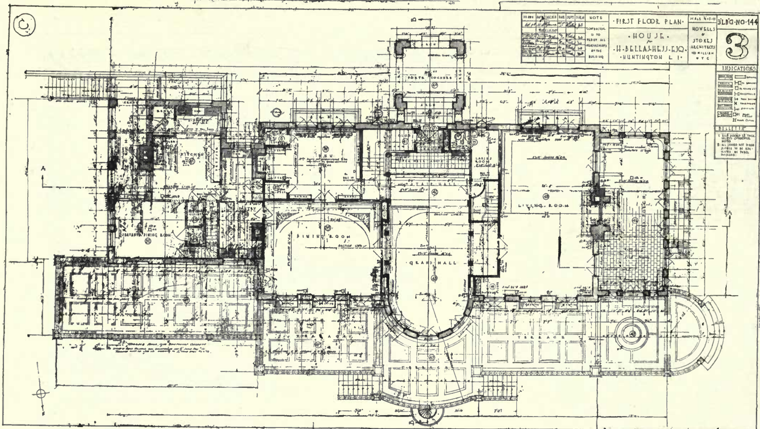
FIG. 64. FIRST FLOOR PLAN—RESIDENCE OF H. BELLAS HESS, ESQ., HUNTINGTON, L. I. HOWELLS & STOKES, ARCHITECTS.
