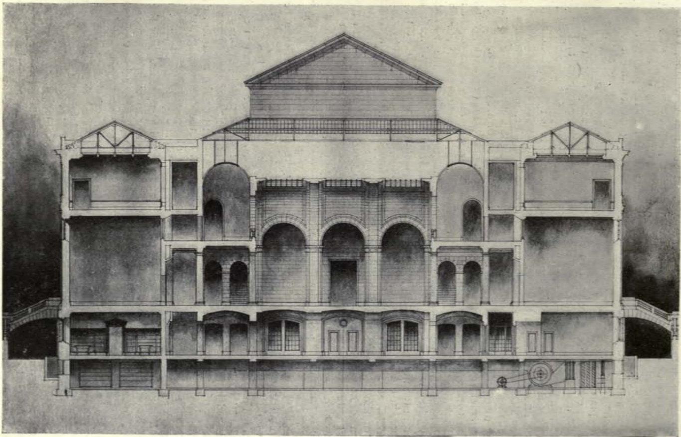
FIG. 5. TRANSVERSE SECTION—DESIGN BY MEYRIC R. ROGERS FOR A SMALL MUSEUM OF ART.
