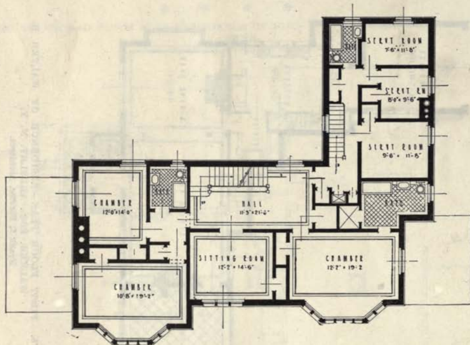
FIG. 78. SECOND FLOOR PLAN—RESIDENCE OF JOHN B. VAN HAELEN, ESQ., HARTSDALE, N. Y. Frank J. Forster, Architect.
