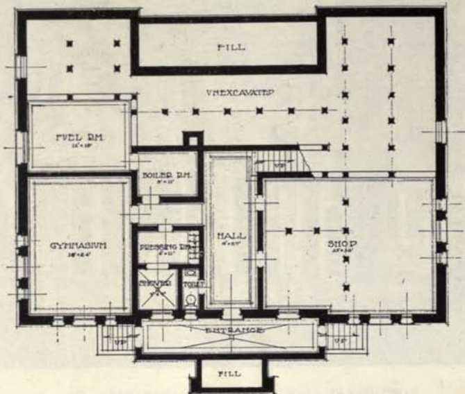
BASEMENT PLAN SCALE 1/8" = 1'-0" SANTA BARBARA COUNTY DETENTION HOME SANTA BARBARA CALIFORNIA
