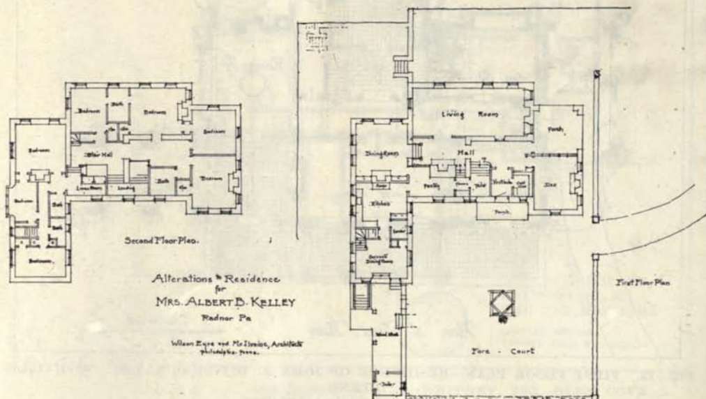
FIG. 72. FIRST AND SECOND FLOOR PLANS—RESIDENCE OF MRS. ALBERT B. KELLEY, RADNOR, PA. Wilson Eyre & McIlvaine, Architects.
