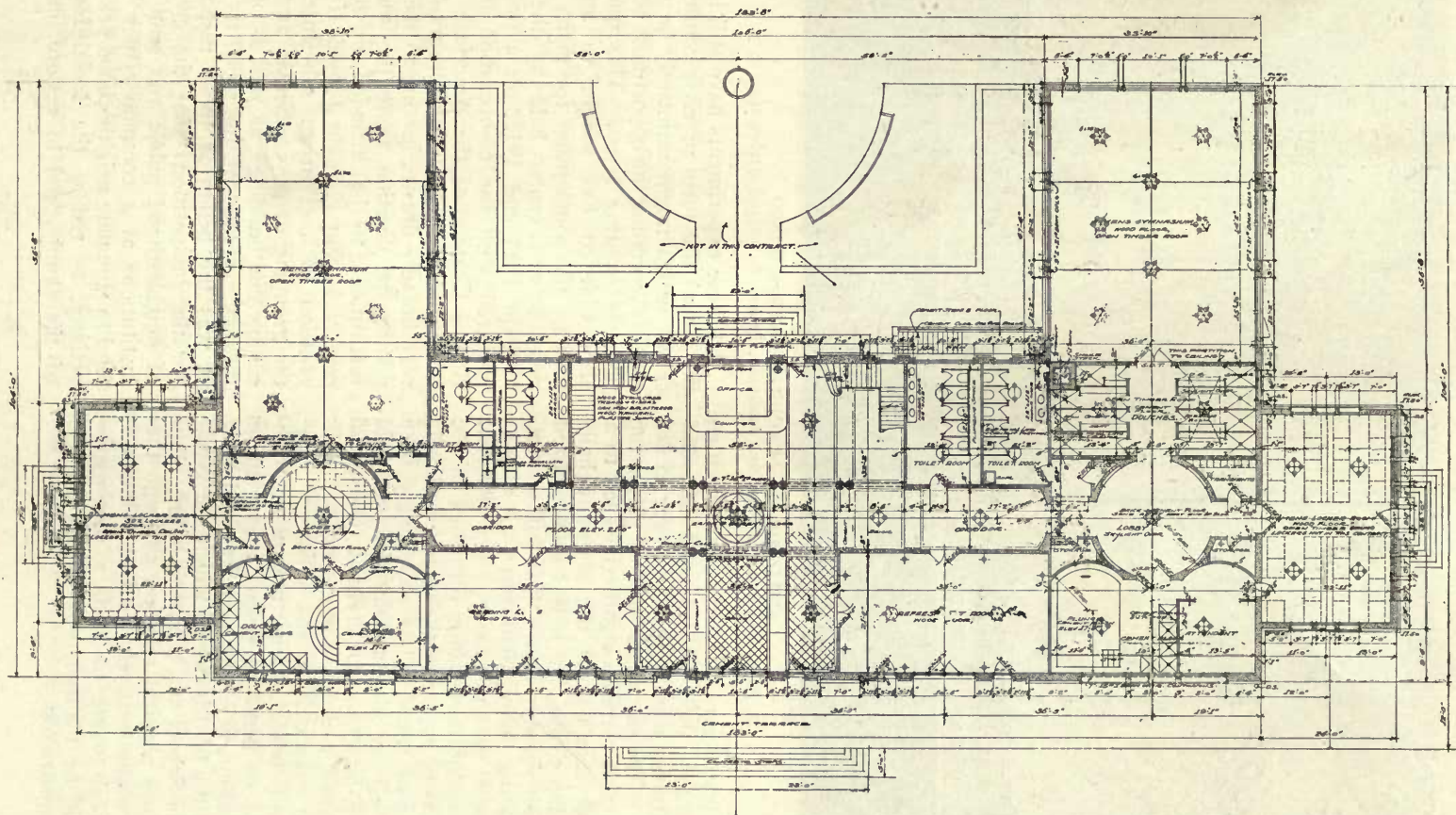
FIRST FLOOR PLAN—SOUTH PARK COMMISSION FIELD HOUSE FOR PARK NO. 9, CHICAGO. D. H. BURNHAM & CO. (GRAHAM, ANDERSON, PROBST & WHITE), ARCHITECTS.
