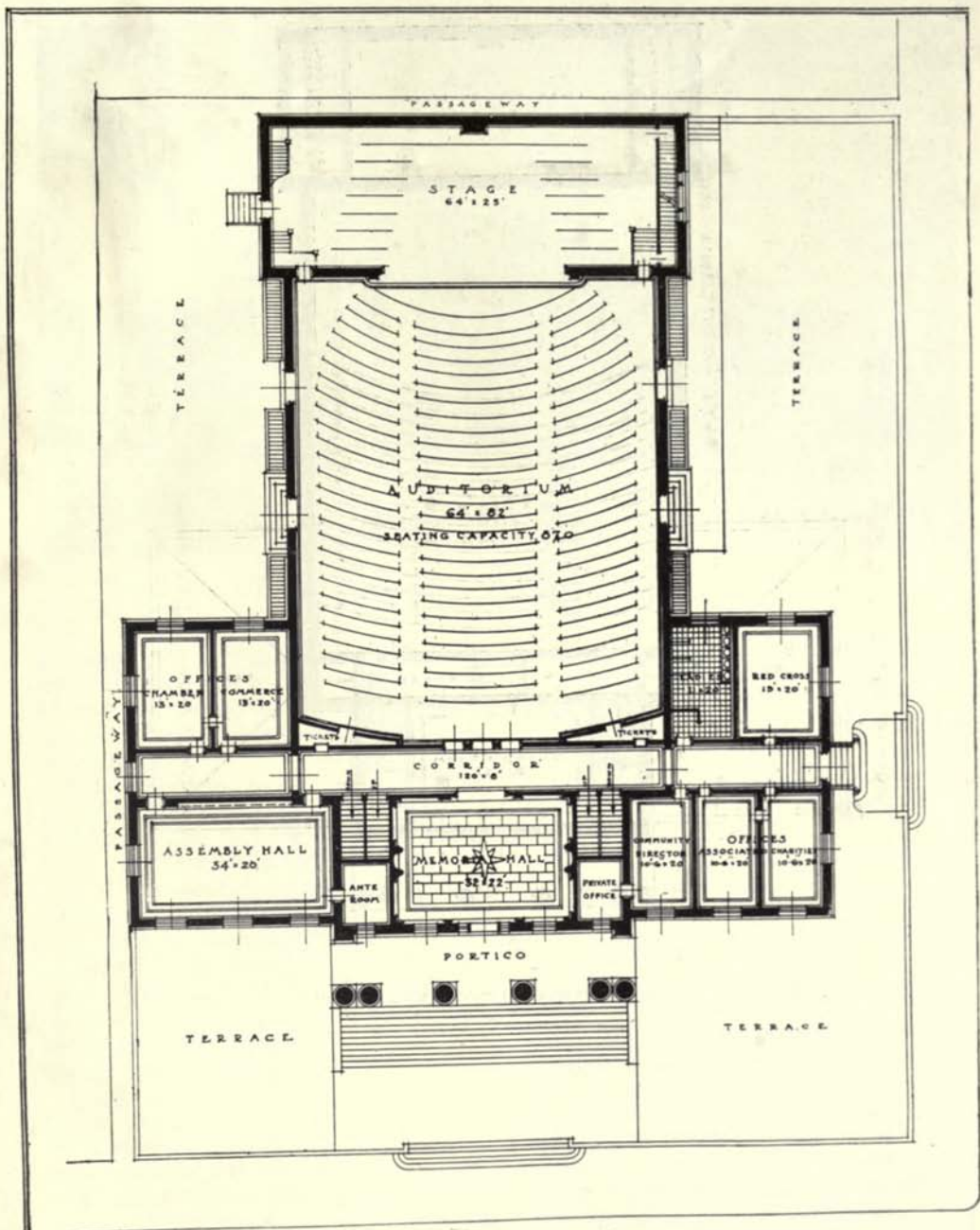
MAIN FLOOR PLAN SCALE 1/8" = 1'-0"
