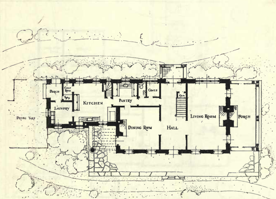
FIG. 68. FIRST FLOOR PLAN—RESIDENCE OF C. E. McINNES, ESQ., RYDAL, PA., Duhring, Okie & Ziegler, Architects.
