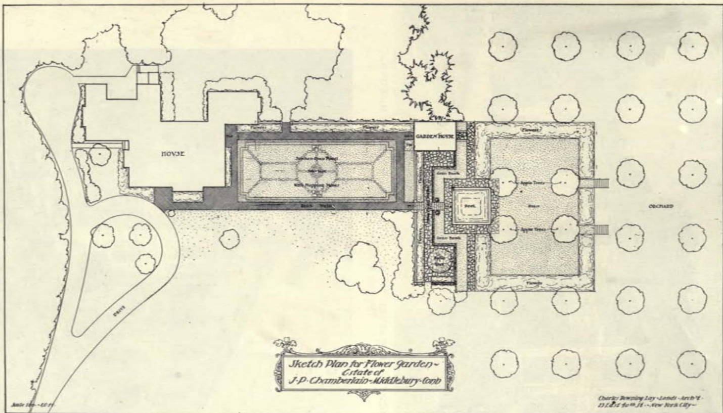
RESIDENCE OF J. P. CHAMBERLAIN, ESQ., MIDDLEBURY, CONN. CHARLES DOWNING LAY, LANDSCAPE ARCHI- TECT; THEODATE POPE, ARCHITECT.
