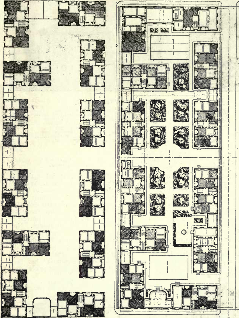
GROUND FLOOR AND SECOND FLOOR PLAN OF ROTTOLE HOUSING DEVELOPMENT, MILAN, BY THE UMANITARIA SOCIETY.
