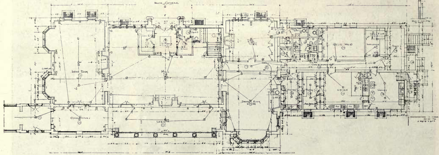
FIG. 18. FIRST FLOOR PLAN—RESIDENCE OF J. WATSON WEBB, ESQ., WOODBURY, L. I. CROSS & CROSS, ARCHITECTS.
