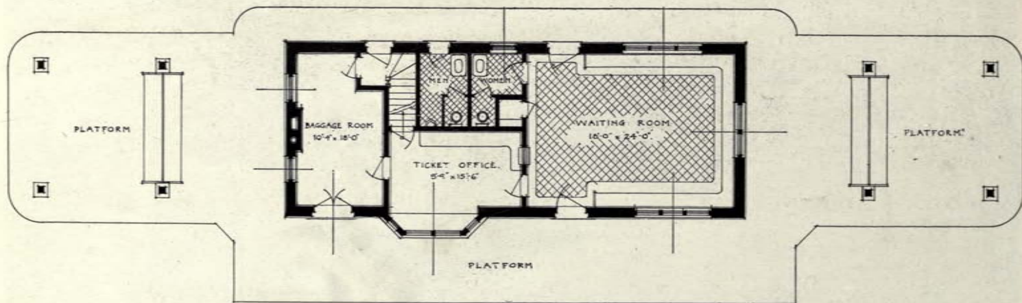
FIRST AND SECOND FLOOR PLANS— RAILWAY STATION AT BALDWIN, L. I. FRANK J. FORSTER, ARCHITECT.
