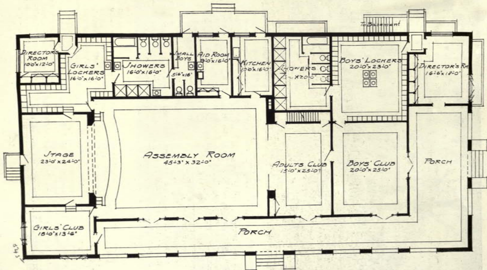
SCRIPPS PLAYGROUND BUILDING, LA JOLLA, CAL. IRVING J. & LOUIS J. GILL, ARCHITECTS.
