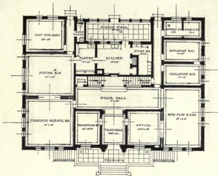
FIRST FLOOR PLAN SCALE 1/8" = 1' SANTA BARBARA COUNTY DETENTION HOME SANTA BARBARA CALIFORNIA
