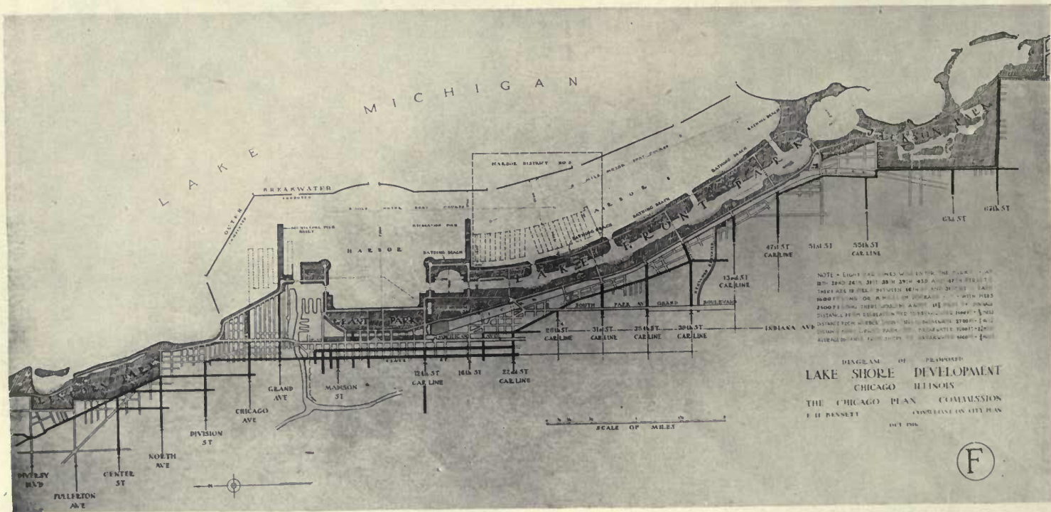
REVISED PLAN FOR LAKE FRONT PARK AND HARBOR DEVELOPMENT BETWEEN GRANT AND JACKSON PARKS: 1,280 ACRES OF PARKS, A FIVE-MILE PROTECTED WATERCOURSE, NINE BATHING BEACHES, PICNIC GROUNDS, MOTOR BOAT COURSES, AND YACHT HARBOR. TAPPED BY TWELVE WEST SIDE STREET CAR LINES.
