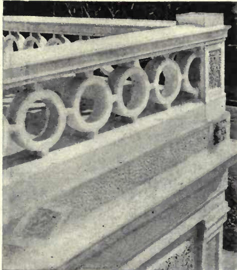
Combination of Smooth Surface Finished With Carborundum Blocks, Pointed Surface, Pebble Dash and Simple Casting Details.
