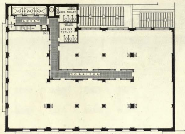
TYPICAL FLOOR PLAN COMMERCIAL NATIONAL BANK BUILDING, WASHINGTON, D. C. Waddy B. Wood, Architect.
