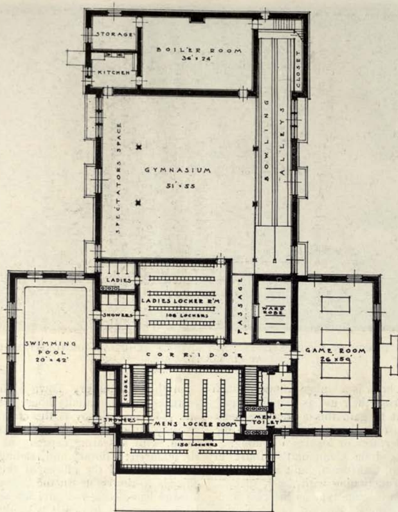
BASEMENT PLAN SCALE \frac{1}{8"=1'-0"}_2
