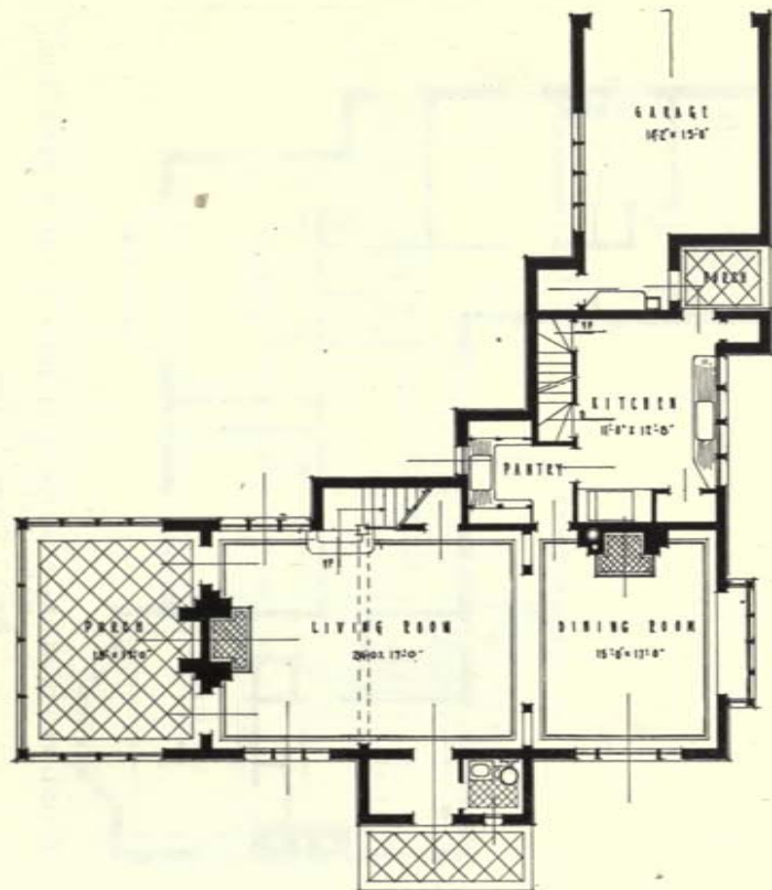
FIG. 75. FIRST FLOOR PLAN—RESIDENCE OF WALTER B. WALKER, ESQ., ARDSLEY, N. Y. Frank J. Forster, Architect.
