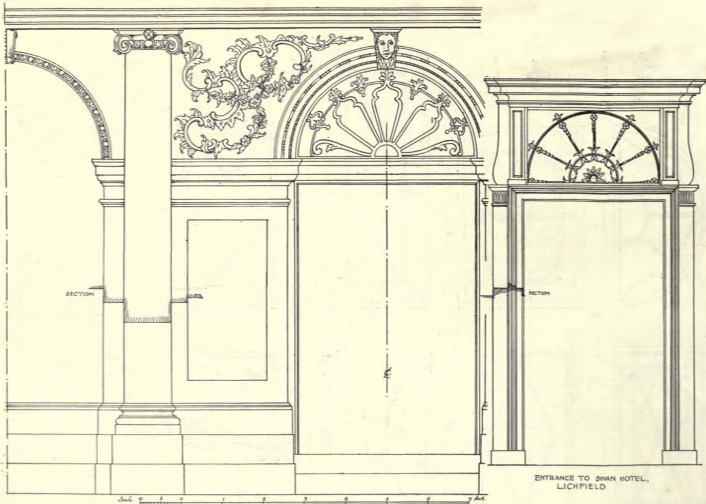
BANK FRONT : HIGH STREET : GUILD FORD.
