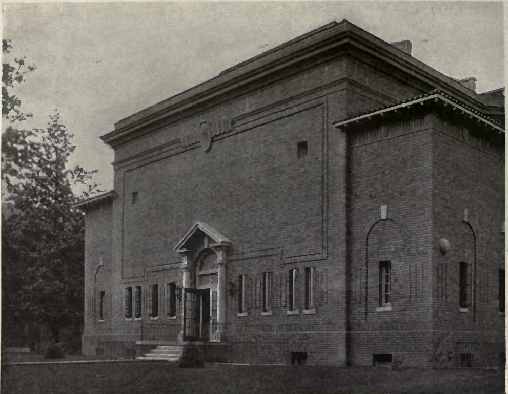
REAR ELEVATION—OGDEN HALL, HAMPTON NORMAL AND AGRICULTURAL INSTITUTE, HAMPTON, VA. Ludlow & Peabody, Architects.
