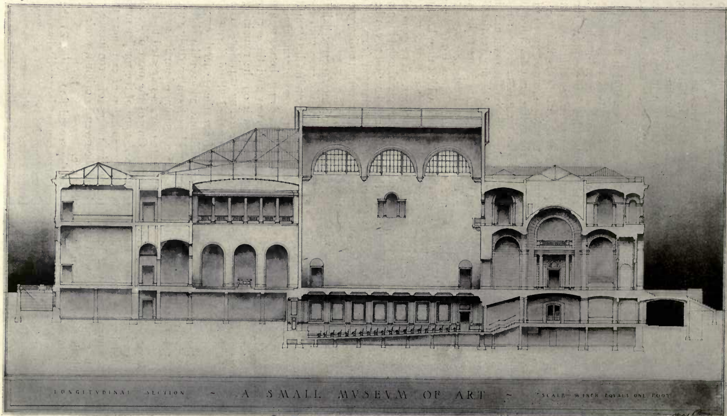
FIG. 4. LONGITUDINAL SECTION—DESIGN BY MEYRIC R. ROGERS FOR A SMALL MUSEUM OF ART.
