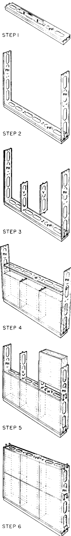
Partitions using Revere's recently developed metal members with Insulux blocks (above) and P-C (below).
