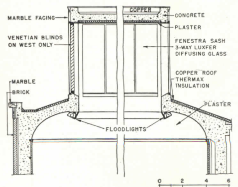
A clerestory of fixed steel sash with special glass daylight the second-floor galleries.
