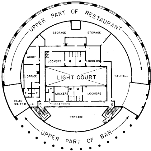
At left, first floor and plot plan, showing the plaza which determined the restaurant's circular shape. On the peak day, 33,400 glasses of beer were served at the main bar. Above, plan of mezzanine shows all rooms facing inward toward light court.
