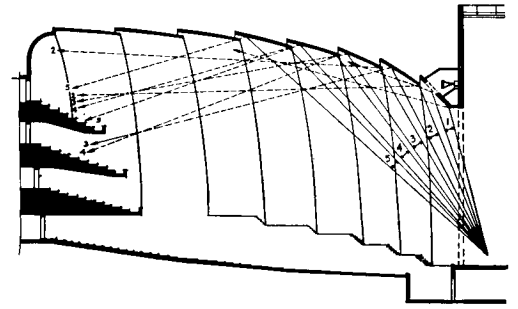
Longitudinal section of Music Hall, Radio City, showing lines of sound reflection from ceiling arches and the spaces for spotlights.
