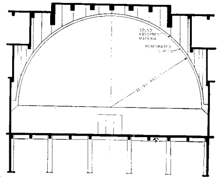
Solution: a perforated-metal screen with absorbent material applied to the main walls back of and above the dome of planetarium.
