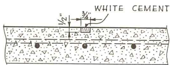
SECTION "A-A" CEMENT CENTER LINE SCALE - 1/2" = 1'-0"
