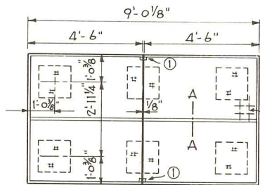
PLAN TABLE TENNIS SCALE - 3/16" = 1'-0"
