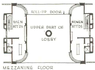
MEZZANINE FLOOR
