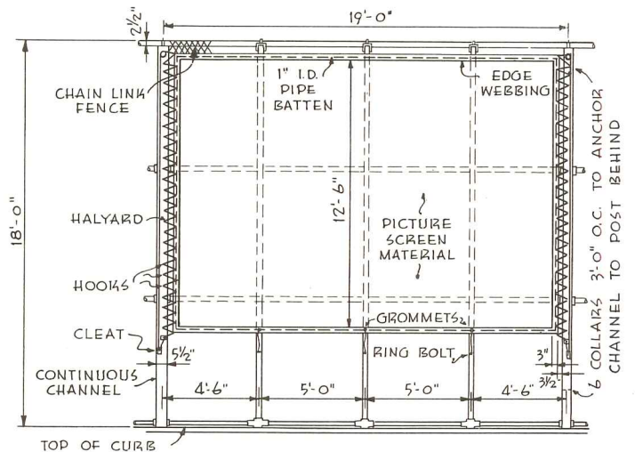
ELEVATION SCALE - 1/8" = 1'-0" PORTABLE MOTION PICTURE SCREEN
