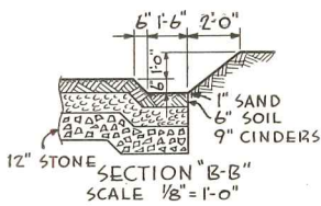
SECTION "B-B" SCALE 1/8" = 1'-0"
