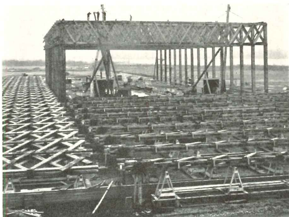
Trusses hoisted into place from trestles on which they were assembled; below, exterior views show assembly portion
