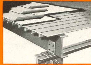
Section of Mahon Steel Roof Deck, as assembled in installation, showing application of insulation and roofing material.
