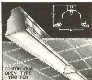
Cross section and installation view of Day-Brite Continuous Single-row Open-type Troffer.
