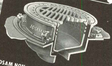
JOSAM GREASE INTERCEPTOR
