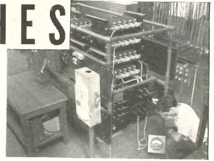
Non-inductive resistance load equipment. For testing higher-rated switches up to 600 Amps., 250 V.
