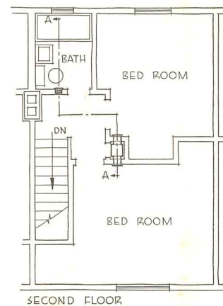
Conservation in the heating system here combines a new "columnar" type of forced air furnace with just about an absolute minimum of duct work. The furnace measures just 26 by 26 in., and has a built-in blower. It is installed in an open closet off the living room, and has a return opening in the bottom, so that no return ducts are necessary. Installed in a defense housing project of the USHA, in Baltimore. Architect, Lucius R. White, Jr.
