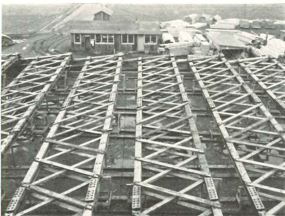
128-ft. timber trusses for a Canadian aircraft plant
