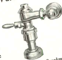
K-9000 BSP - Speakman "SI-FLO" Closet Flush Valve with Back-Syphon Preventer.
