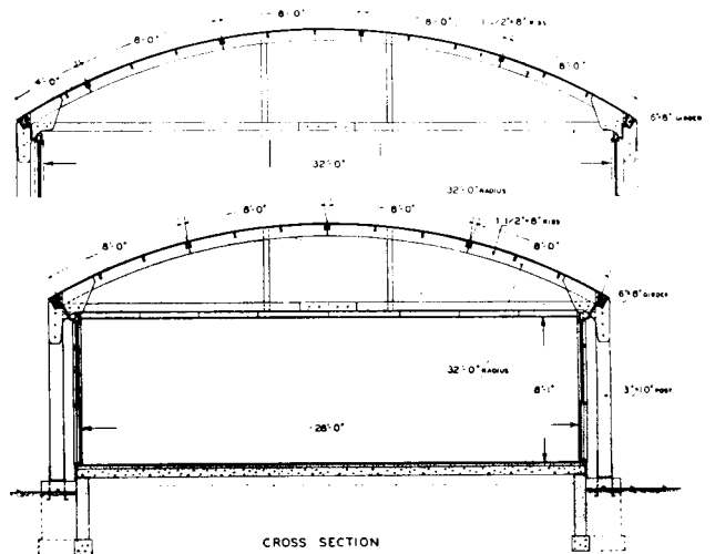
CROSS SECTION
