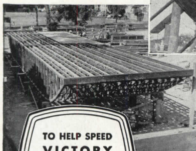
● (Above) The bottom skin of these Higgins lighters consists of (from left) outer planking, a layer of thoroughly water-proofed canvas and an underlay of 5/8-inch Exterior-type Douglas Fir Plywood. The Higgins Industries use vast quantities of plywood in the many types of auxiliary vessels they are building.
