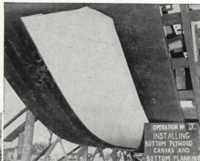
● (Above) The bottom skin of these Higgins lighters consists of (from left) outer planking, a layer of thoroughly water-proofed canvas and an underlay of 5/8-inch Exterior-type Douglas Fir Plywood. The Higgins Industries use vast quantities of plywood in the many types of auxiliary vessels they are building.
