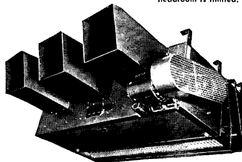
CARRIER TYPE 46 R HEAT DIFFUSING UNIT —for economical heating and ventilating of large enclosures. Designed for horizontal suspension from ceiling or truss-work, floor-mounting, or vertical suspension.
