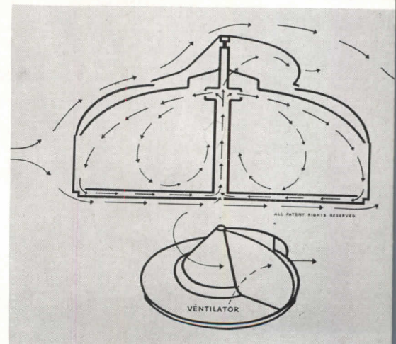
Top, plan showing room divisions, revolving closets, "ovolving" shelves, and interior bath units. Center, cut away section showing supporting rings and cables and living room interior. Bottom, arrows show wind flow outside and "fountain" flow of warmed, conditioned air throughout the interior of the house
