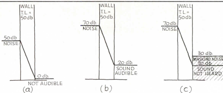
Fig. 2. Reduction of sound through an insulating partition
