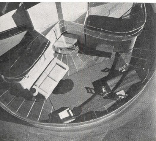
The Fuller House model. Top, plexiglas windows do not support roof as walls (and floor) are hung from rings by cables running to central mast. Center. Looking down into the bedrooms, closets and interior baths. Bottom. Looking down into living room; balconies add space over kitchen and entrance hall; see plan
