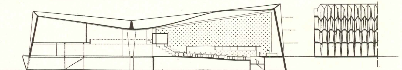
Conference Building: longitudinal section and details of end walls, which furnish part of roof support
