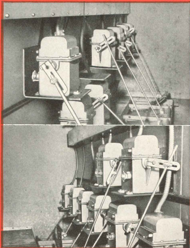
Banks of Proportioning Control Motors—Job included one motor which contained a 37000 to 1 gear reduction, also quantities of two-position and reversing control motors.
