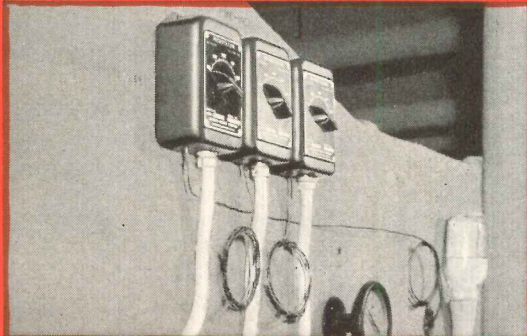
Motor-operated valves (above) and remote bulb thermostats (below)—typical of the over 400 Barber-Colman electric components used for temperature control in Research Tower.
