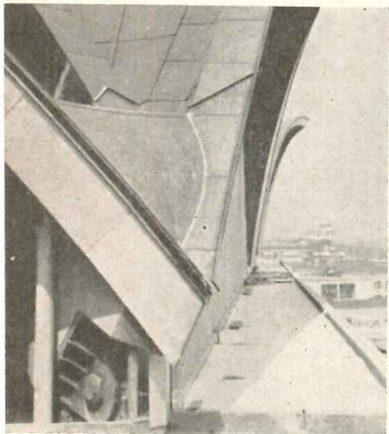
One of the hinges, four per dome, which carry the shells; under construction and with finish completed
