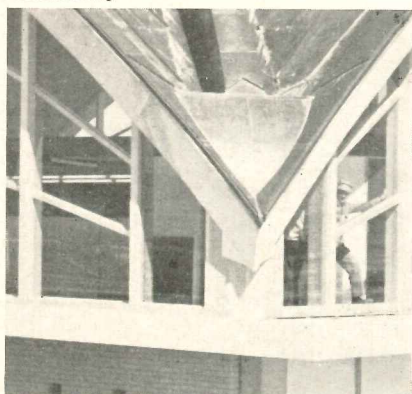
One of the hinges, four per dome, which carry the shells; under construction and with finish completed
