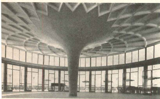
A highly expressive geometric pattern was formed in the ceiling of this restaurant designed by A. La Padula through a refinement in Nervi's pre-fabrication techniques. Precast, coffered sections, about 1-in. thick were assembled on a platform with spaces left between for reinforcing of the stiffening ribs
