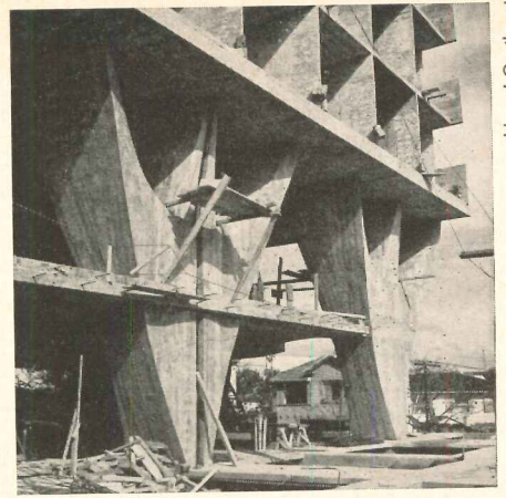
Construction detail. Niemeyer
