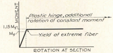
Moment-Rotation Diagram for WF Beam
