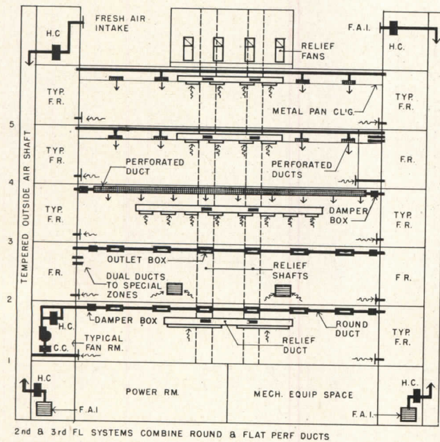
2nd & 3rd FL SYSTEMS COMBINE ROUND & FLAT PERF DUCTS
