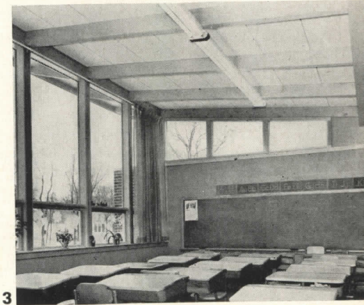
1 , Macomber's standardized framing elements with simplified connections, West Cedar Elementary School, Waverly, Iowa; Perkins & Will, Architects. 2 , Universal space-frame structure, school in Wayne, Mich.; Sun Chien Hsiao, designer; Charles W. Atwood, Architect and Manufacturer. 3 , Wood post-and-beam structure, preformed roof planking, Cedar Heights Grade School, Cedar Falls, Iowa; Thorson, Thorson & Madson, Architects (R. R. Blanch photo). 4 , Arches and thin shells for large, unobstructed areas, Union Station Junior High School, Napa, Calif.; Corlett & Spachman, Architects (P. Palmer photo)
