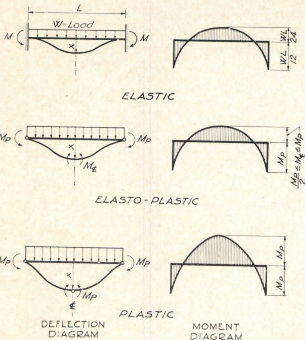
Redistribution of Moments for Fixed End Beams
