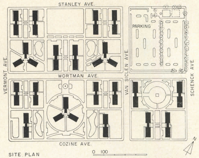
Site plan closes four of six cross streets, develops extensive open areas for playgrounds and lawns and parking. Buildings will cover 12 per cent of ground. Model photograph (below) is in effect a sun and shadow diagram, showing placement of buildings to avoid shading
