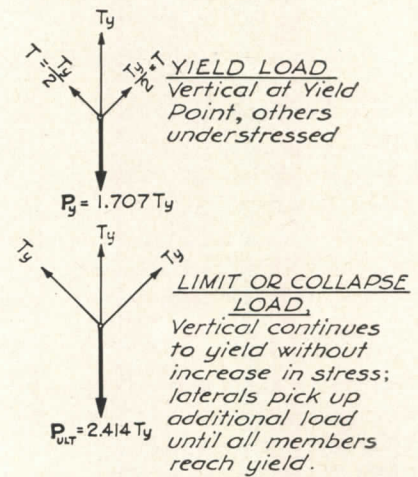
Limit Analysis for a Simple Indeterminate Truss
