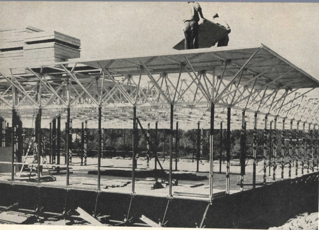
5: Space-frame
