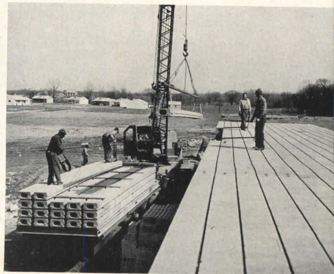
23: Concrete, Rapidex lightweight preformed slabs
