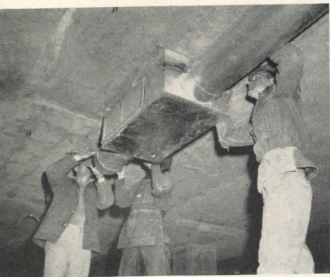
Airtight fit is made between outlet box and duct by connectors and strap
