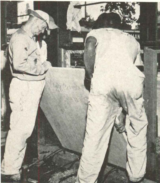
Prefabricated limestone: (1) a "thru-wall" unit with 3-in. limestone, 2-in. cellular glass, 3-in. waste stone; (2) window surround with 1-in. stone, 3-in. insulation and sprayed aggregate
