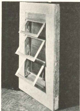
Prefabricated limestone: (1) a "thru-wall" unit with 3-in. limestone, 2-in. cellular glass, 3-in. waste stone; (2) window surround with 1-in. stone, 3-in. insulation and sprayed aggregate
