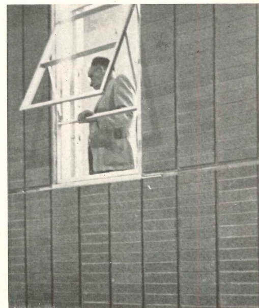
High strength mortar makes possible a prefabricated panel wall of brick, 15 to 20 high and two wide
