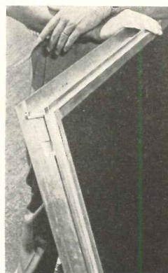
Marble curtain wall panel uses 1/2-in. marble slab backed up by insulation and composition board, all held by an aluminum frame which interlocks with other frames. It weighs 9 lb per sq ft
