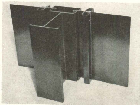
Positioning of exterior vertical I beams, spandrels and T bars at wall line
