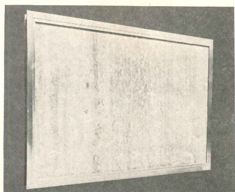
Marble curtain wall panel uses 1/2-in. marble slab backed up by insulation and composition board, all held by an aluminum frame which interlocks with other frames. It weighs 9 lb per sq ft
