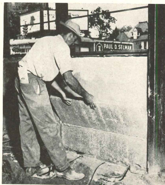
Marble curtain wall panel uses 1/2-in. marble slab backed up by insulation and composition board, all held by an aluminum frame which interlocks with other frames. It weighs 9 lb per sq ft
