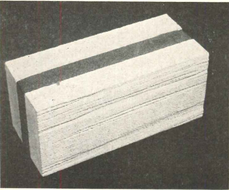
Prefabricated limestone: (1) a "thru-wall" unit with 3-in. limestone, 2-in. cellular glass, 3-in. waste stone; (2) window surround with 1-in. stone, 3-in. insulation and sprayed aggregate
