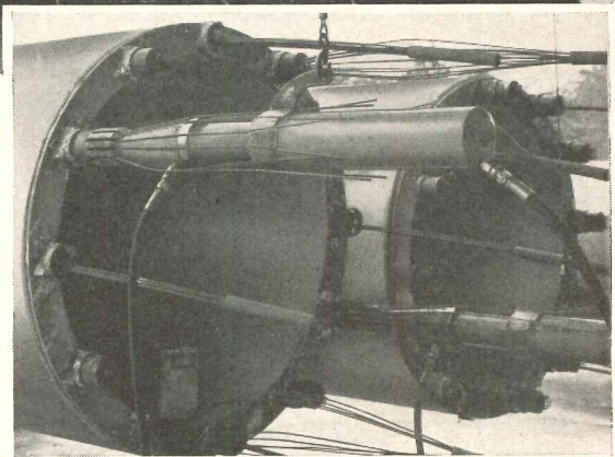
Post-tensioning the cables. Piles are 54" outside diameter, 80 and 96 feet long, and stressed with 12 cables each containing 12 wires, .192" in diameter.
