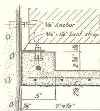
Detail of anchoring at vertical surround
