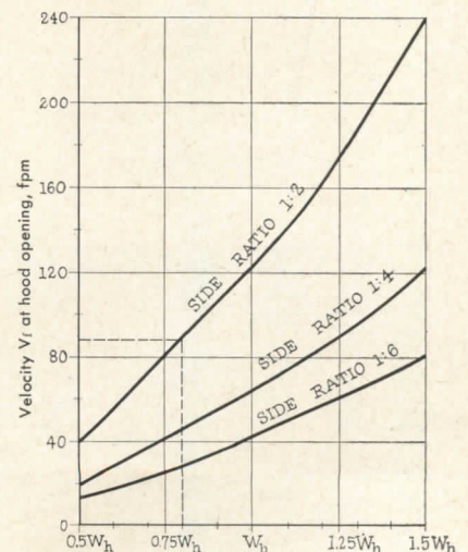
X (in Terms of W_h ) for Rectangular Shed Type Hoods
