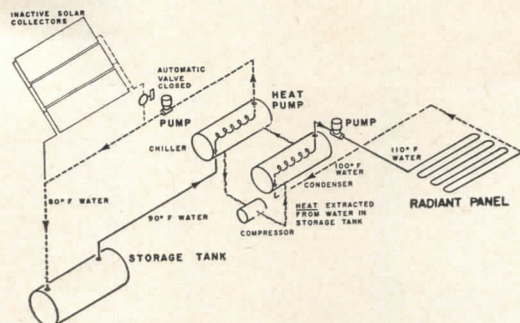
During extended dark days, heat pump heats building. Heat pump can also be used for summer cooling, with cooled water from chiller going directly into radiant system and extracted heat being discharged to the outside through evaporative water cooler
