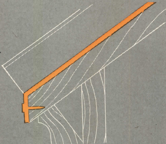
EDGE STRIP DETAIL BATTEN SEAM ROOF Fig 1
