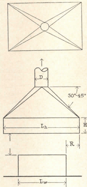
Freely Suspended Hood
