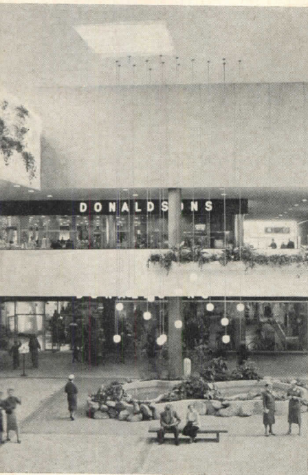
The Garden Court, 109 by 270 ft, acts as a plenum chamber to supply 70 F ventilation air to Dayton's store and tenant stores. Air enters
