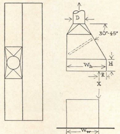
Shed Type Hood
