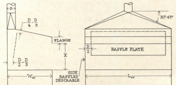
Lateral Exhaust (Enclosing Hood Type)
