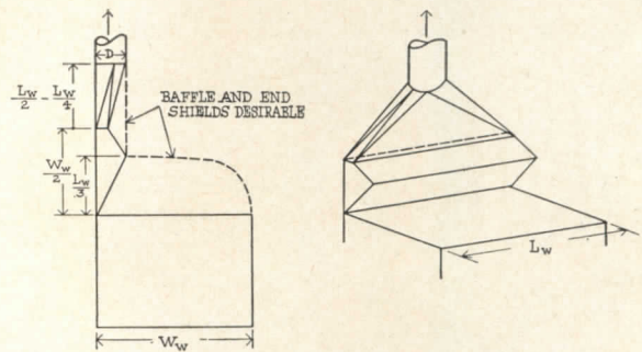
Lateral Exhaust (Rear or Side Draft)
