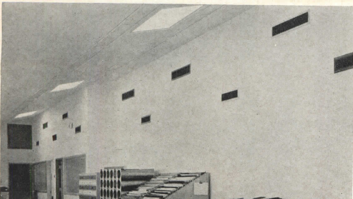
South wall separates office space from equipment room. Light from skylights bounces off wall and lights room
