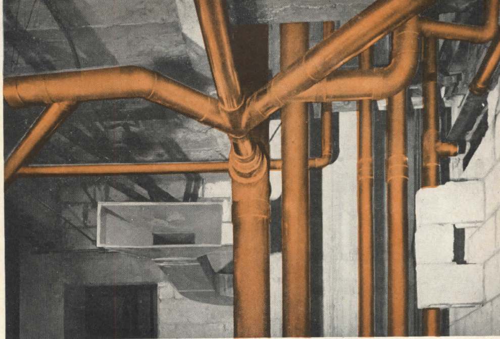
Save space and weight in all buildings—even skyscrapers. Copper tubes in main pipe shaft of a 43-story office building. Copper tube saves space because pipe shaft and furred spaces at columns and ceilings can be smaller. Light weight speeds installation.
