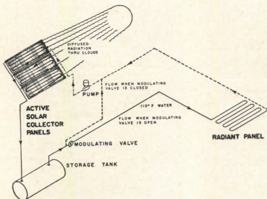
When modulating valve is open, 110F to 140F water from collectors flows directly through tank to heating system. When it is closed, water circulates from collectors to tank, storing heated water. Then cooled water can be used in the radiant panels
