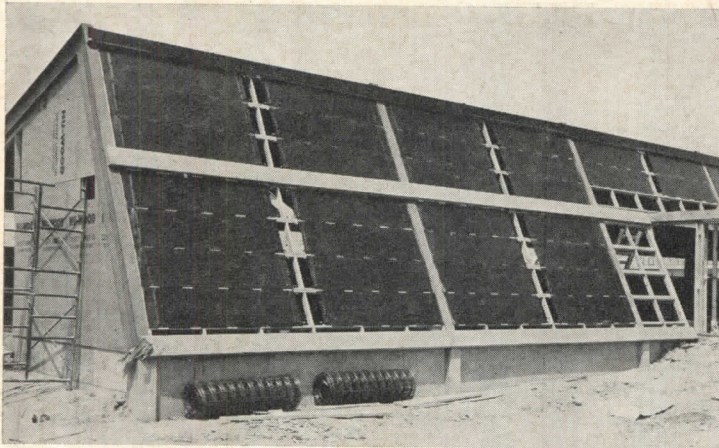
Black aluminum collector panels enclose integral water channels \frac{1}{2} in. wide by \frac{1}{8} in. deep
