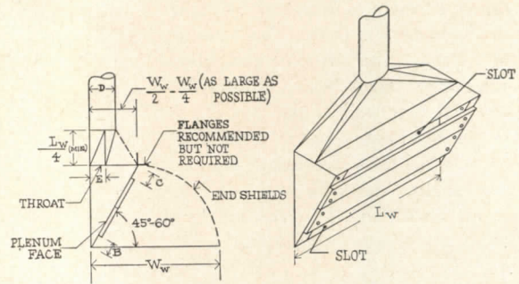
Lateral Exhaust (Slant Type)
