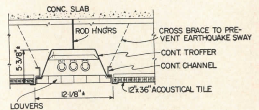
Continuous fluorescent troffers hung from floor slab support ceiling tiles
