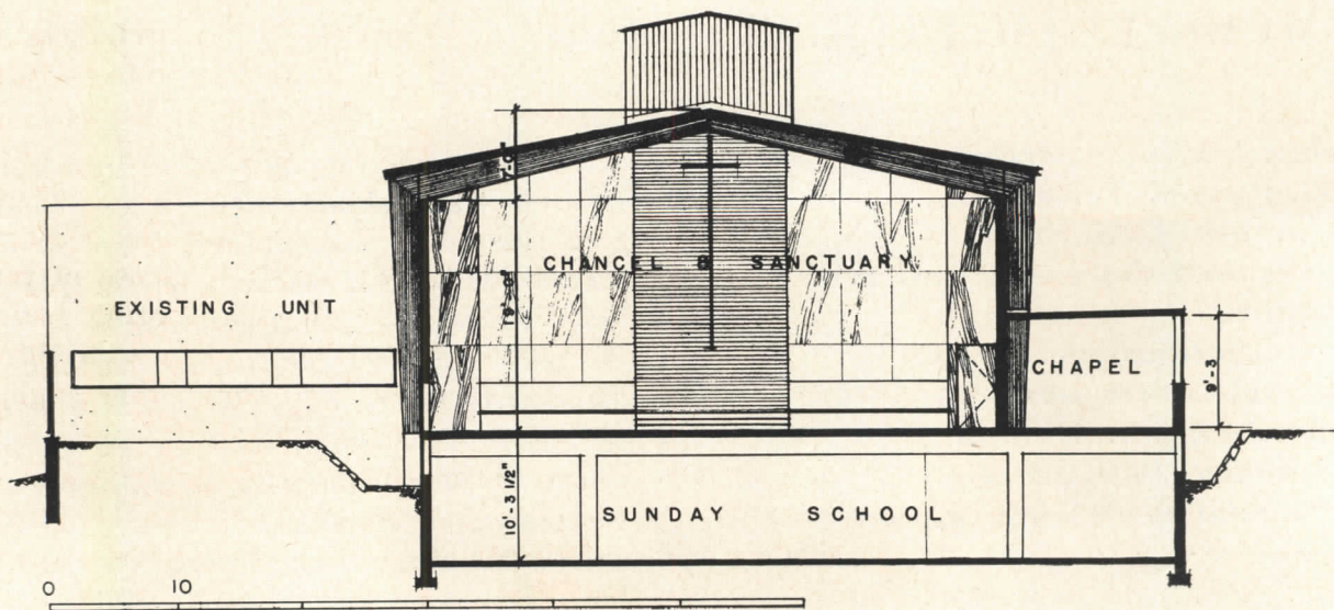
LATERAL SECTION
