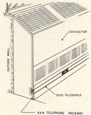
Continuous electrical plug-in strip and telephone raceway are recessed in bottom of perimeter convectors
