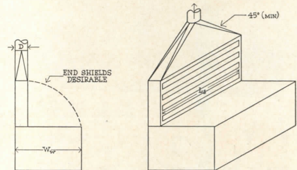
Lateral Exhaust (Slot Type)
