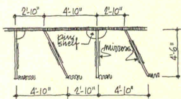
TYPICAL FITTING ROOM
