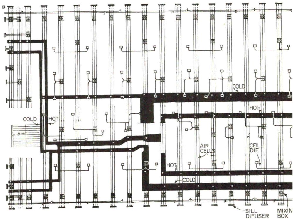
Mechanical Plan
