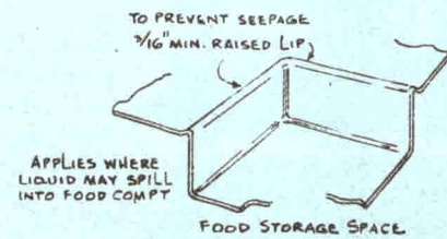
3.055 — TOP OPENING OR RIM
