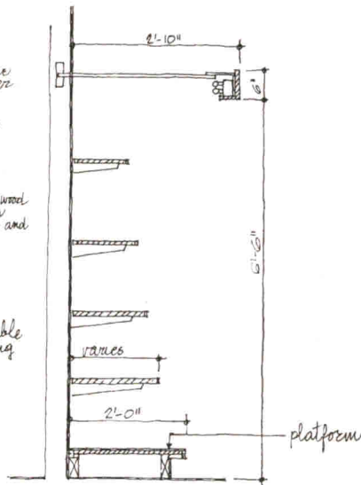
BACK FIXTURE with SHELVES only
