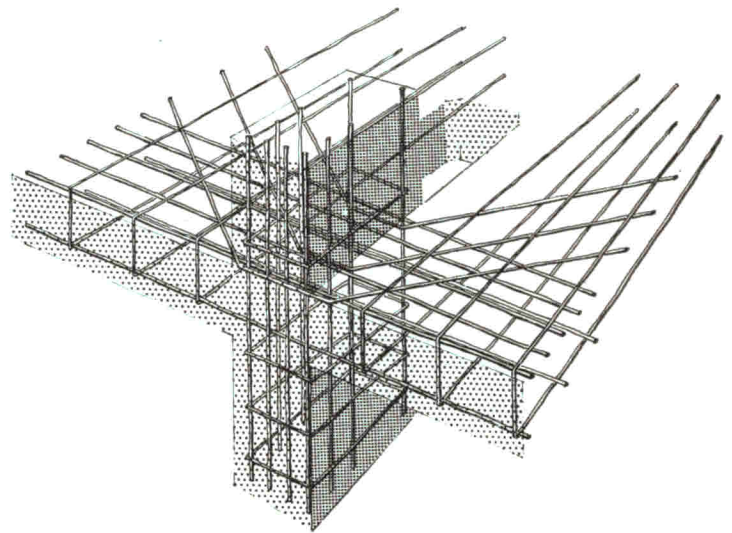
Figure 11. This schematic diagram indicates how reinforcement might be arranged to prevent the failures shown by keeping stresses within the capacity of the concrete. To simplify the drawing, general reinforcement of the slab is not shown
