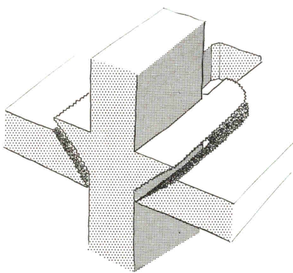
Figure 8. The familiar "diagonal Tension" failure of a flat plate, failure due to tensile stresses along a plane at 45 degrees to the planes of maximum shear, can be prevented by using diagonal reinforcing bars or vertical stirrups
