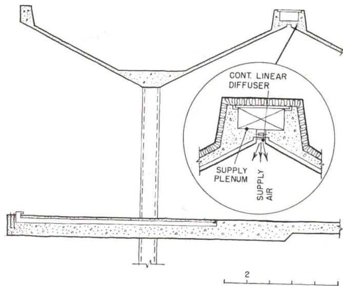
Above: Top floor of the Service Building (center in photo previous page) has a roof of inverted concrete umbrellas which cover the cafeteria and kitchen. Air supply for the cafeteria comes from plenums up to 68-ft long formed by the top edges of the umbrellas. Air supply for the corridor around the perimeter of the building is delivered through a plenum provided in the top of the floor slab.
