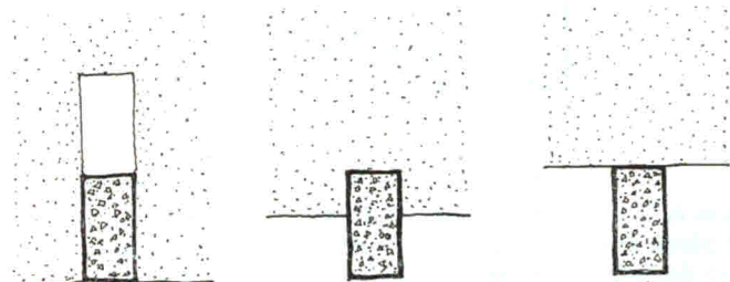
Figure 7. Careful analysis and detailing makes it possible to take advantage of the design implications of column connections like these
