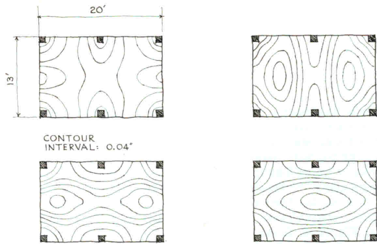
Figure 4. "Contour maps" of the deflections in a flat plate slab show the variations caused by varying the reinforcing steel
