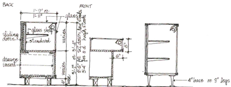
SHOWCASE - wood frame
