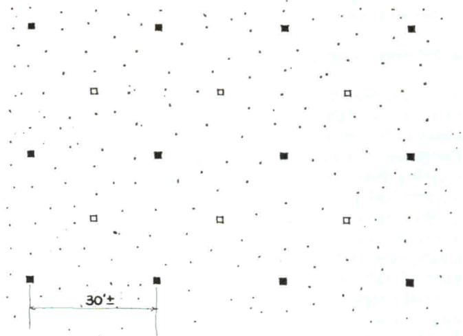
Figure 5. Introducing center "prop" columns prevents excessive deflections in long spans without increasing the thickness of the slab
