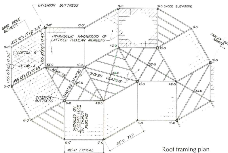
Roof framing plan
