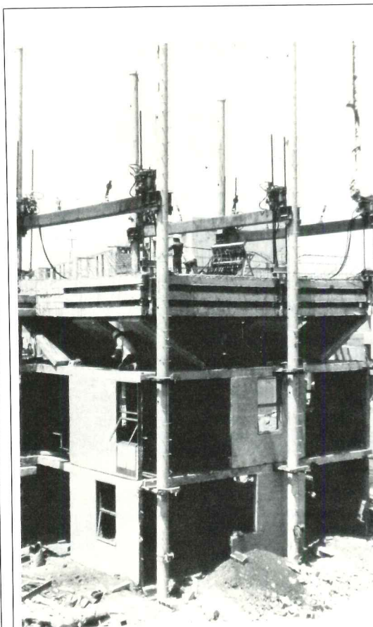
Above: Cortina System in erection
