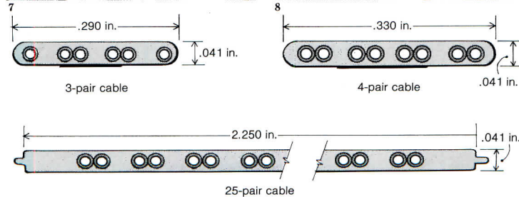
TELECOMMUNICATIONS CABLE
