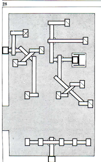
Photo 27: typical flat wire installation for power, telephone and data, Thomas & Betts; figure 28: computer-generated layout for power, telephone and data produced on a system comprising a Prime CPU, a Hewlett Packard 7580A pen plotter and modified Medusa software, AMP; figure 29: layout illustrating the principle of through-receptacle wiring and variable-angle cable bends, Thomas & Betts.
