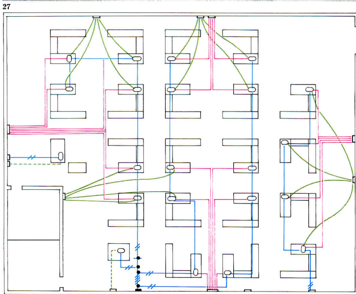
Photo 27: typical flat wire installation for power, telephone and data, Thomas & Betts; figure 28: computer-generated layout for power, telephone and data produced on a system comprising a Prime CPU, a Hewlett Packard 7580A pen plotter and modified Medusa software, AMP; figure 29: layout illustrating the principle of through-receptacle wiring and variable-angle cable bends, Thomas & Betts.
