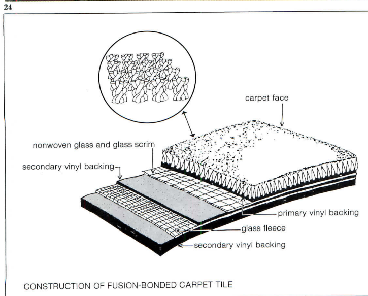
Photo 24: model P5300 Series fusion-bonded carpet tiles over flat telephone cable, installed at AMP Inc., Schaumburg, Illinois, Interface Flooring Systems; figure 25: construction of fusion-bonded carpet tile, Interface; photo 26: fusion-bonded carpet tiles, Milliken & Company.
