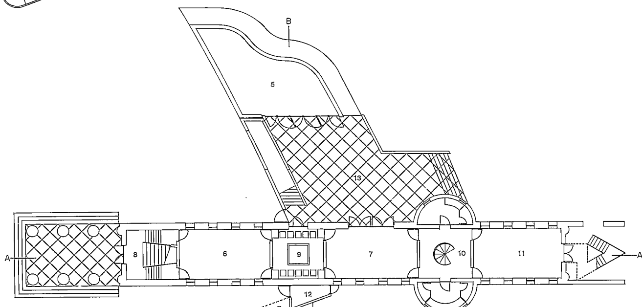
FIRST FLOOR
