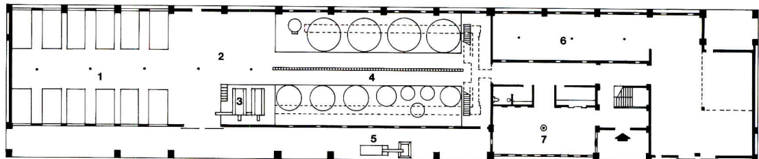
GROUND FLOOR
