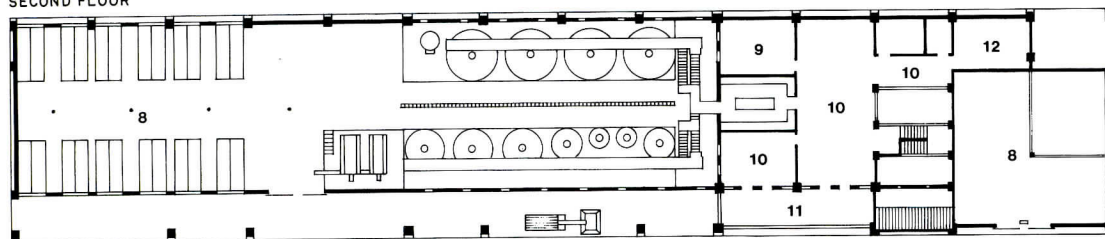
SECOND FLOOR
