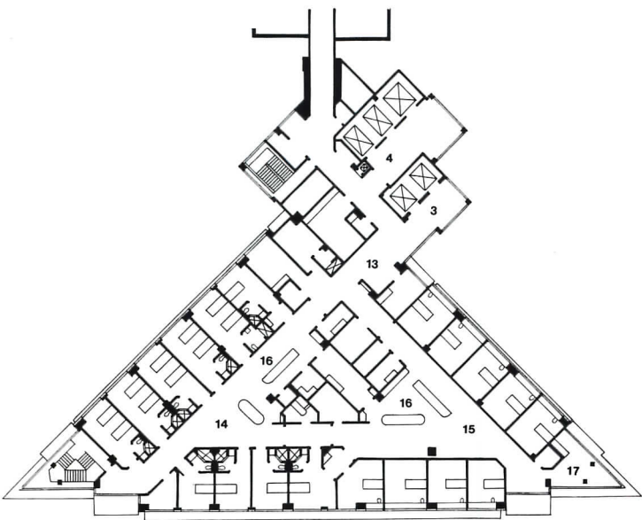
SECOND FLOOR (3 AND 4 SIMILAR)
