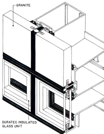
Horizon system with stone.
