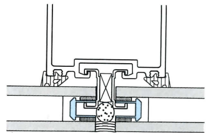
Plan view of Duratec unit, showing Structural Spacer.
