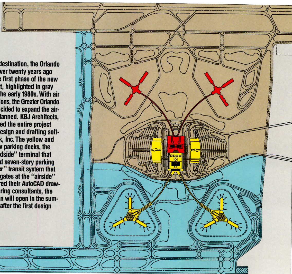
The new airside building features wings arrayed at 120-degree angles to handle a large variety of aircraft. AutoCAD was used to draw the different planes and to check how they would fit the building and surrounding aprons.
