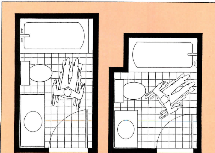
Standards for bathrooms are typical of what opponents of the new HUD guidelines dislike. While minimal builder bathrooms have contained 37.5 square feet, the HUD bathroom (left) would increase that to 51 square feet. But the opponents' version (right) would only require 43 square feet and allow more wheelchair maneuverability.
