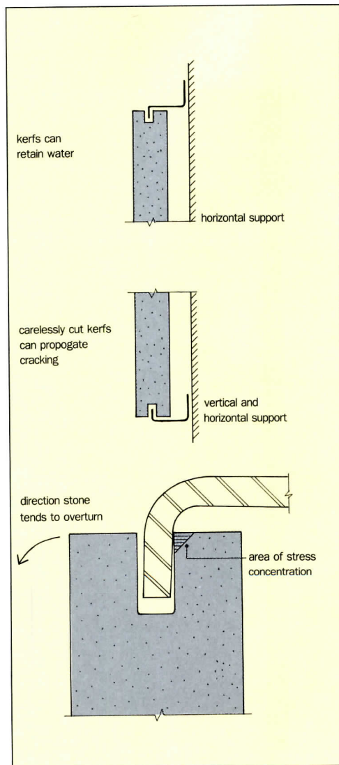
The absorption of a given type of stone (Table 3, top) and the design of kerfs (above) both affect whether the facade will trap water.
