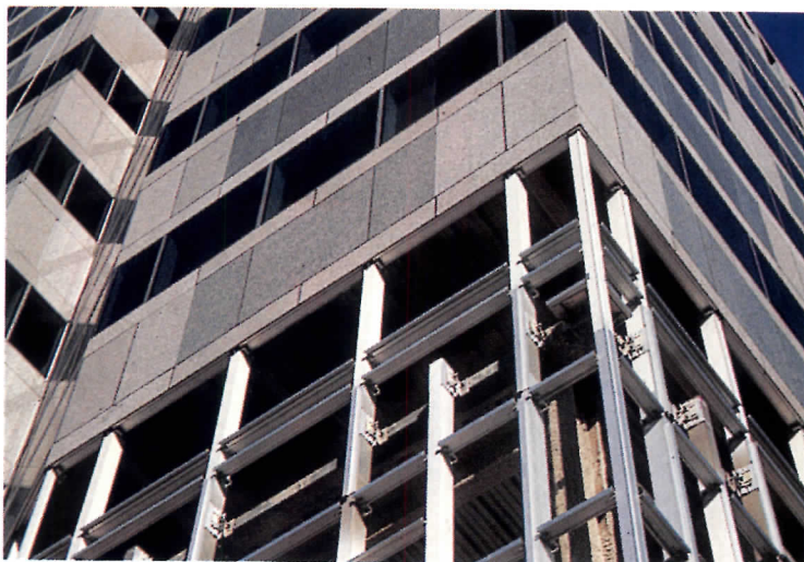
Erection of thin-stone panels at Commerce Square, Philadelphia. Pei Cobb Freed & Partners, Architect.
