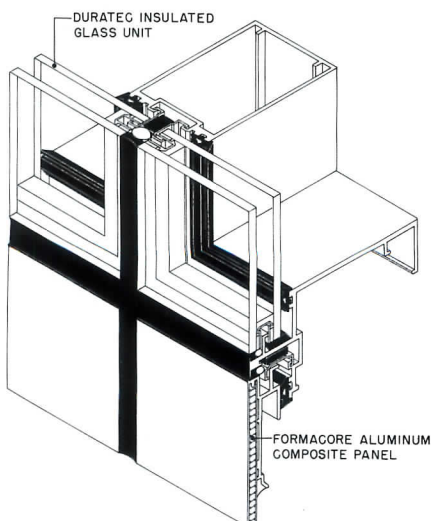
Horizon with metal core panel.
