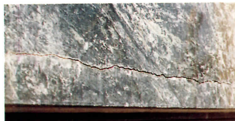
Stone damaged by differential movements: at a connection (top left), above a window (bottom left), and pavement over a structural slab (above).
