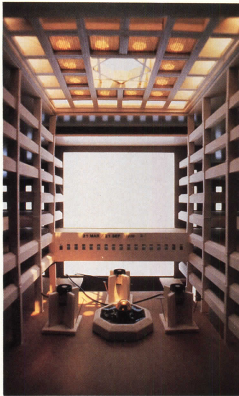
Sensors on the floor of the model measure the incoming light. In the background, an unobtrusive note labels the photograph so the designer can later compare conditions for a variety of times of the day and the year.
