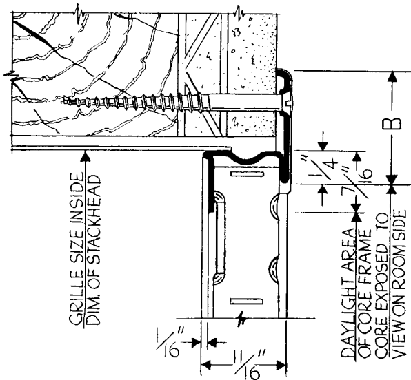
DETAIL OF SIDEWALL GRILLE — FULL SCALE DIM. "B" = 7/8" ON MODEL "EA"; 1 1/4" ON MODEL "EB"
