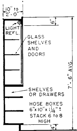
SECTION HOSIERY, HANDBAGS
