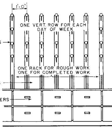
SECTION WALL CASES for WORKROOMS
