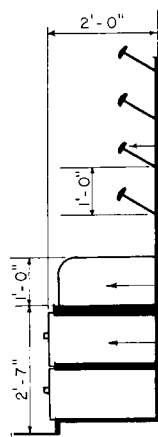
SECTION WALL CASES for WORKROOMS
