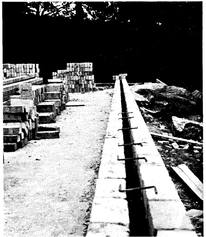
Fig. 5. Moisture penetration is eliminated, strength unimpaired by Cavity Wall construction. Tied by \frac{1}{4} -in. steel rods, outer 4 in. serves as surfacing, inner carries load.
