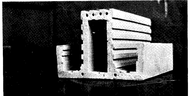
Fig. 5. Moisture penetration is eliminated, strength unimpaired by Cavity Wall construction. Tied by \frac{1}{4} -in. steel rods, outer 4 in. serves as surfacing, inner carries load.
