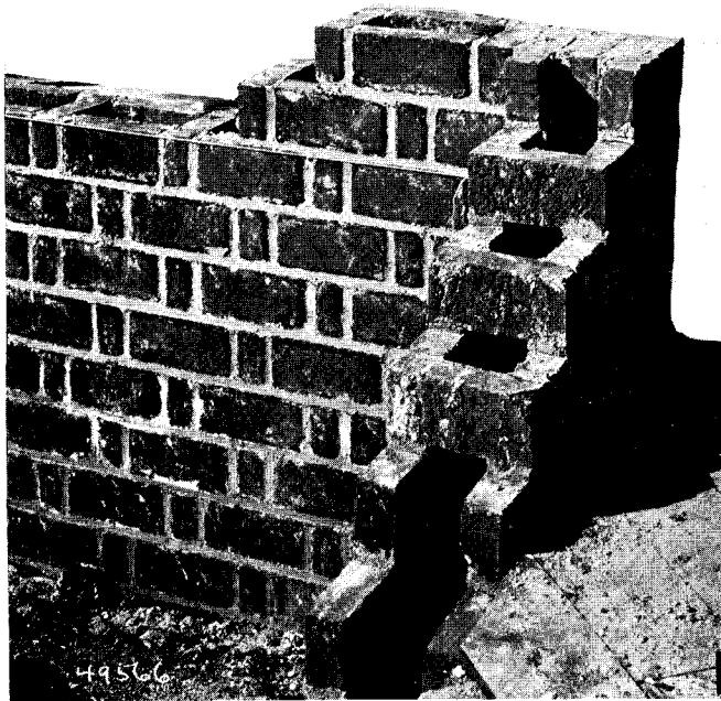
Fig. 4. Simplest of all advances in ordinary brick masonry is this hollow wall construction. Although boasting some advantages, moisture can still penetrate via headers.
