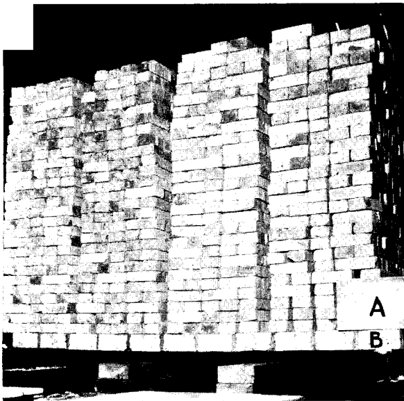
Fig. 1. Reinforced brick slab, 3 3/4 in. by 2 ft. 8 in. by 8 ft. 0 in., with load of 397 lbs. per sq. ft. Reinforcing members are six 3/8-in. round bars placed longitudinally 1/2 in. from bottom of slab.
