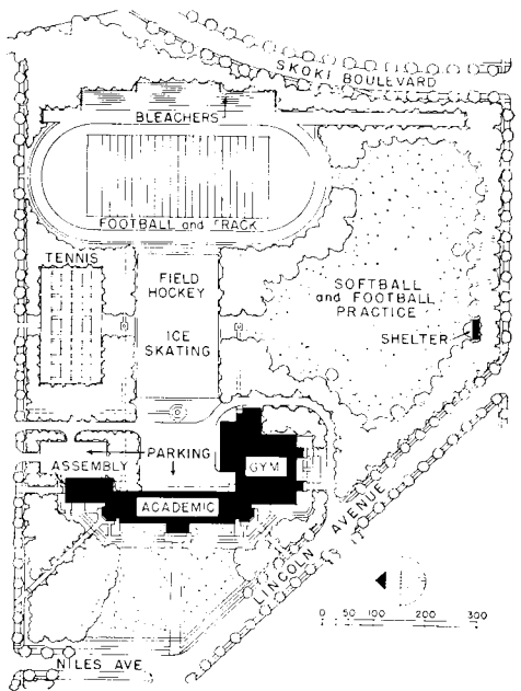
Plot plan
