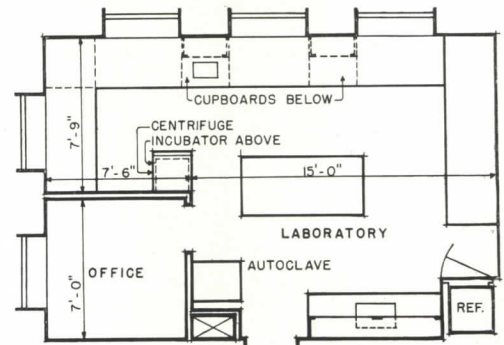
Above, typical laboratory developed for a 200-bed hospital, and, at right, similar provisions for a 50-bed hospital. Both plans were developed from sketches prepared by H. A. Bliss.
