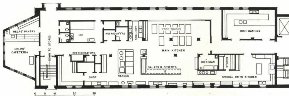
Kitchen, Washington Co. Hospital (200 beds), Hagerstown, Md.; Buckler and Fenhagen, architects.
