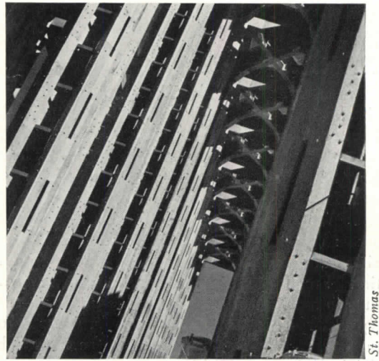
Fig. 8. Columns built up of timber and plywood.
