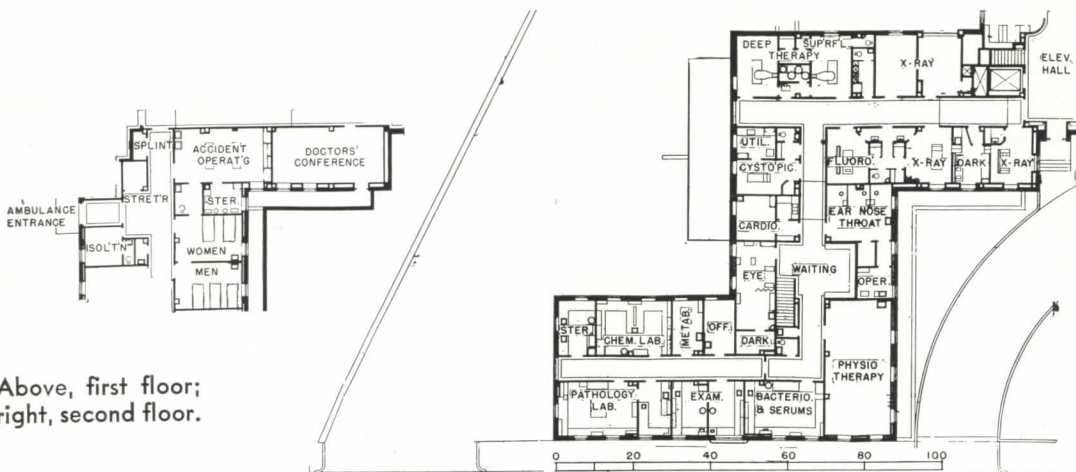
Part of the clinical facilities at White Plains Hospital, White Plains, N. Y.; Schultze and Weaver, architects. Included here are emergency, or casualty, unit; laboratories; physiotherapy room; X-ray department; and several specialized treatment rooms. Operating, delivery, pharmacy, and morgue provisions are elsewhere in the building.
