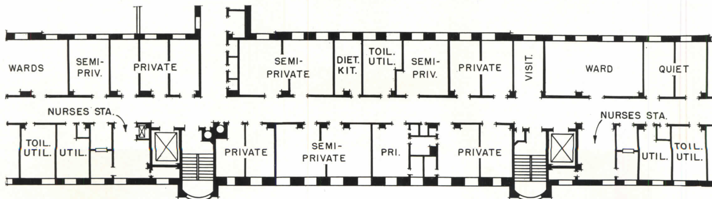
Method of combining wards, rooms, and service rooms in Rome Hospital, Rome, N. Y.
