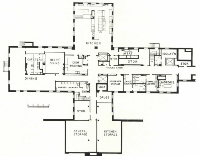
Service basement, Sheboygan Memorial Hospital, Sheboygan, Wis.; Schmidt, Garden, and Erikson, architects; E. A. Stubenranch, associate architect. In this case, laundry is done outside the building.
