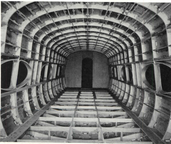
Fig. 3. As structure—wood and plywood.
