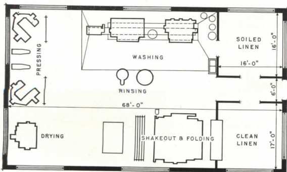
Plan of typical laundry for a 100-bed hospital.
