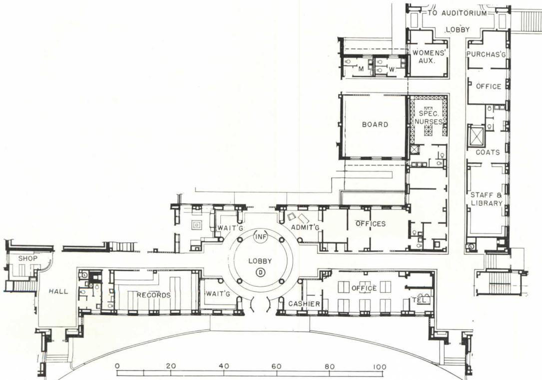
Administrative areas, first floor, White Plains Hospital, White Plains, N. Y.; Schultze and Weaver, architects.
