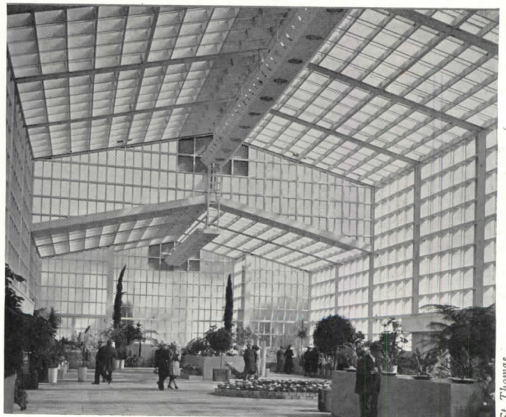
Fig. 4. As framing—all plywood.
