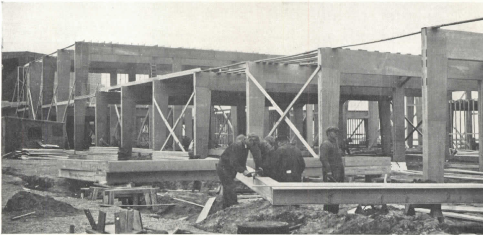
Fig. 11. Plywood nailed to a rigid frame forms extremely strong, lightweight members.
