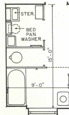
Standard plan, bedpan-bath unit, makes the seldom-used patients' bath do double duty.
