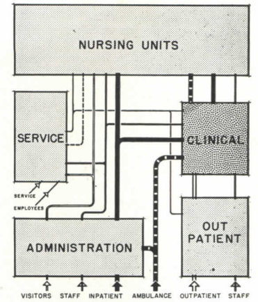
Diagram at left shows spaces and circulation necessary for clinical services; key above relates clinical departments to remainder of hospital.
