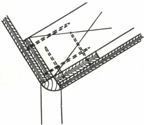
Construction detail of an outside corner
