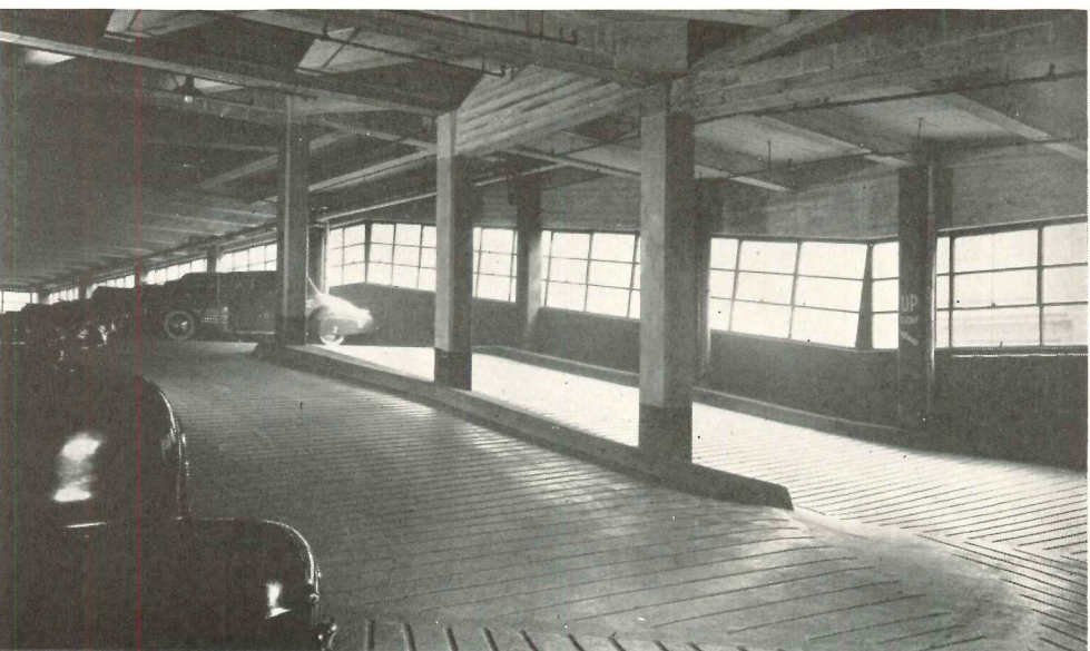
PSF PARKING GARAGE, PHILADELPHIA, PA.; HOWE and LESCAZE, ARCHITECTS. This garage, with shops on the first floor, almost achieves the “open” construction suggested above.
