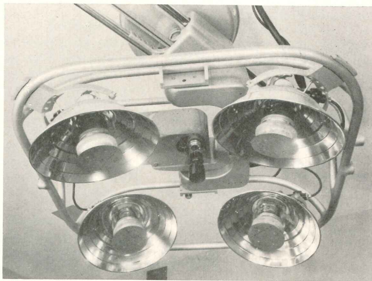
Closeup of fixture shows how camera is mounted in light frame. Lamps are special color-balanced units, designed to permit best possible color
