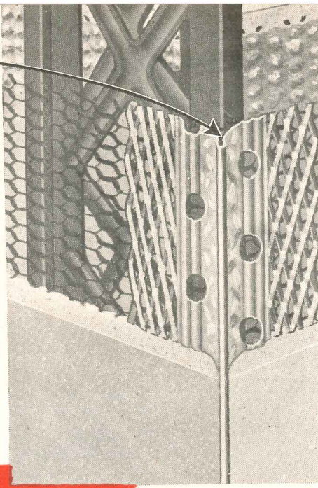
Firesafe construction at best: improved Milcor Super-Ex Corner Bead, Milcor Mesh Lath, and Milcor Steel
