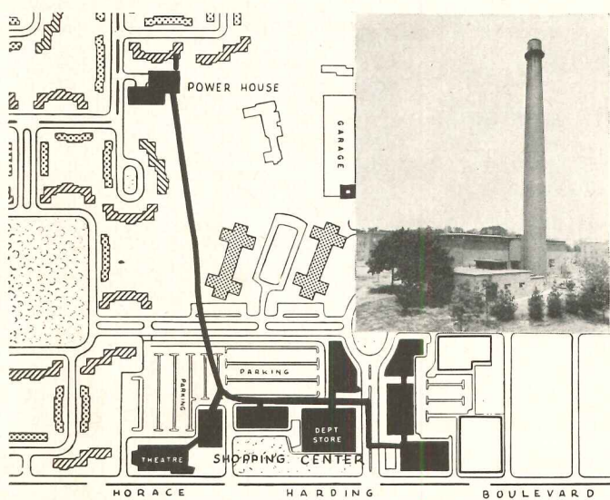
Diagram shows layout of modern shopping center at Fresh Meadows, Long Island, N. Y. Note location of power house (inset) and chilled-water lines from central plant to group of buildings in foreground.
