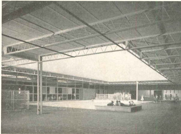
Donald Barthelme & Associates: West Columbia, Tex., Elementary School, 1952
