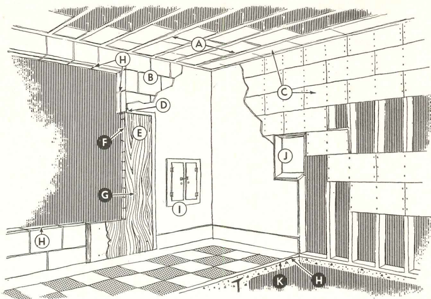
Above: cover of new X-ray accessories catalog. Right, room equipped with X-ray protective materials: A, lead insulated furring bars; B, lead insulated blocks; C, lead insulated lath; D, lead insulated frame; E, lead insulated door; F, cast lead fasteners; G, face veneer; H, lead overlap; I, lead insulated film cabinet with lead insulated flange; J, operators' window with lead frame and speaking opening
