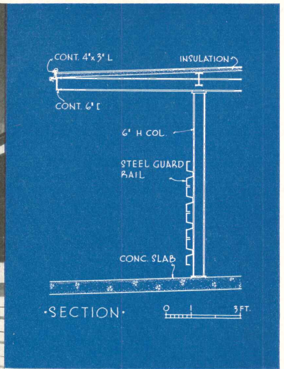
Steel guard rail at concourse and stair to observation deck are painted fire-engine red; copings and signs are porcelain enamel. Below: de-planed passengers and baggage meet under cover on north side
