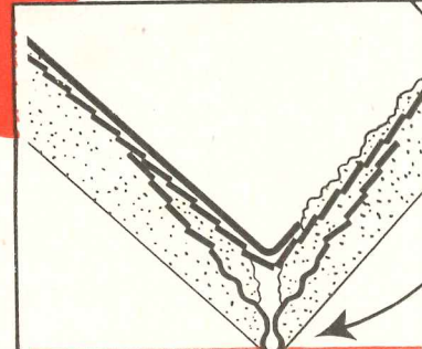
Here's why Super-Ex corners are so long-lasting: note greater depth of plaster adjacent to bead area . . . spring fit adapts easily to any specified depth plaster ground — whether it be 3/4", or 1/2" . . . and solid metal that protects corner at point of greatest strain.
