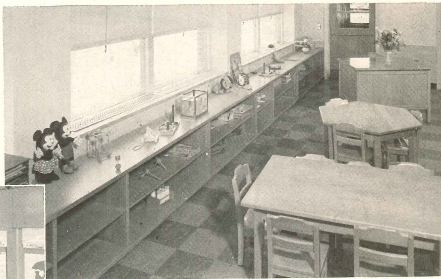
Above: Kindergarten of the Lafayette School. Here concealed Webster System Radiators deliver heat through top outlet grilles shown in window sills. Air enters below toy shelving.
