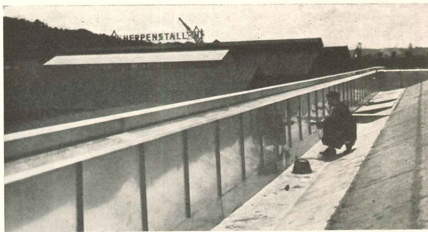
Above: the parapet cover is conventional except that it forms an outlet for exhaust air. Both parapet cover and parapet are of stainless steel. Left: stainless roof panels were placed over felt
