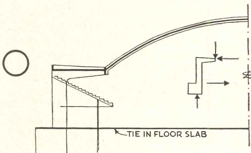
BUTTRESS WITH HORIZONTAL CANTILEVER
