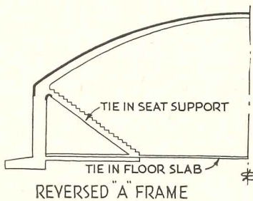
REVERSED "A" FRAME
