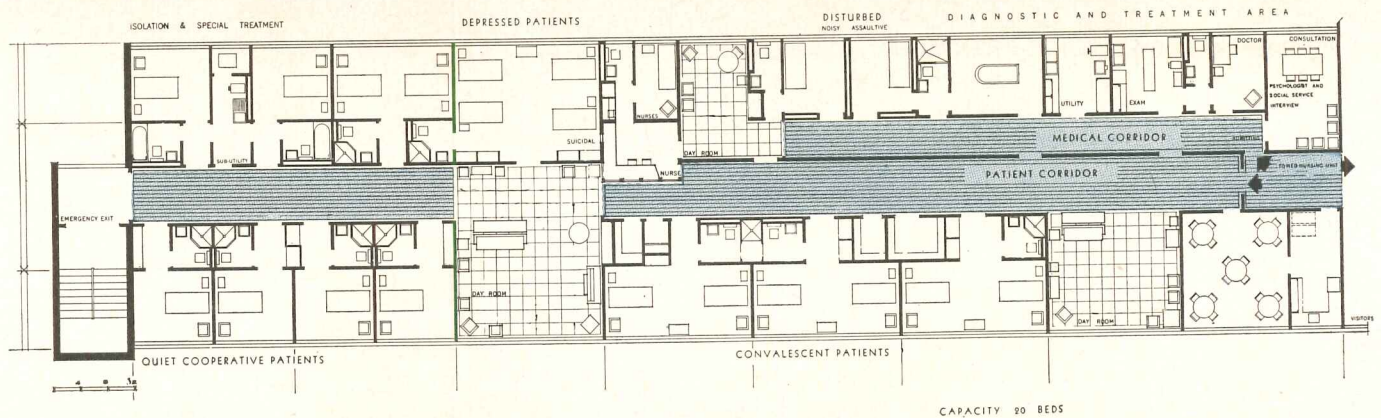
SUGGESTED PLAN OF PSYCHIATRIC WARD FOR THE GENERAL HOSPITAL
