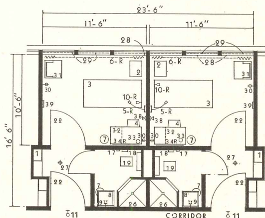
Plan No. 3. PRIVATE SPECIAL TREATMENT ROOMS
