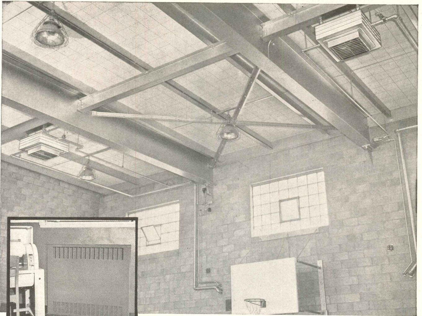
Webster-Nesbitt Down-Blow Unit Heaters up in the air, out of the way, provide heat for the gymnasium. Up in the air and along the wall, also out of the way, are the Webster Series "26" Traps draining the units. Left: Webster Type E Convector alongside ironer in home economics department. The metal front is finished in a bright contrasting color.
