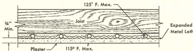
1 | In one typical installation of panel heating systems with gypsum plaster, the metal lath is placed below the heating elements. This type of installation requires only the standard plaster thickness of 3/4 in., but the plaster keys partially surround the heating elements
