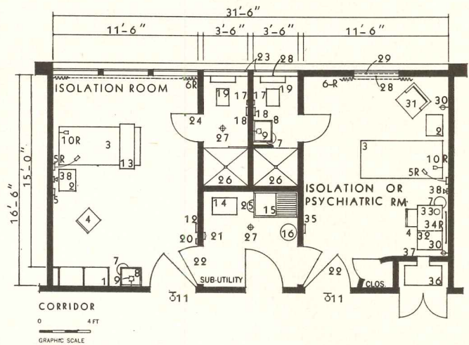
Plan No. 1. ISOLATION AND PSYCHIATRIC ROOMS
