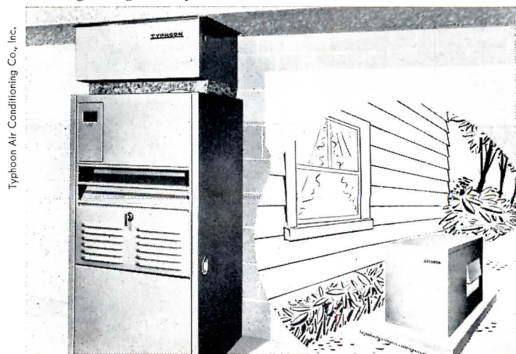
Cooling coils go above furnace, condenser outside in conversion unit
