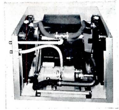
Automobile-type radiators cool condenser water for 3-hp conditioner
