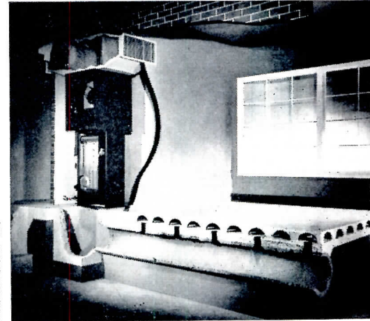
Double-deck floor slab for panel heating
