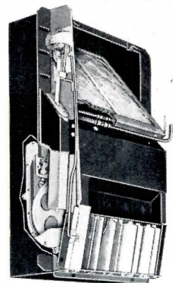
Steam serves as heating medium and drives fan as well in room units
