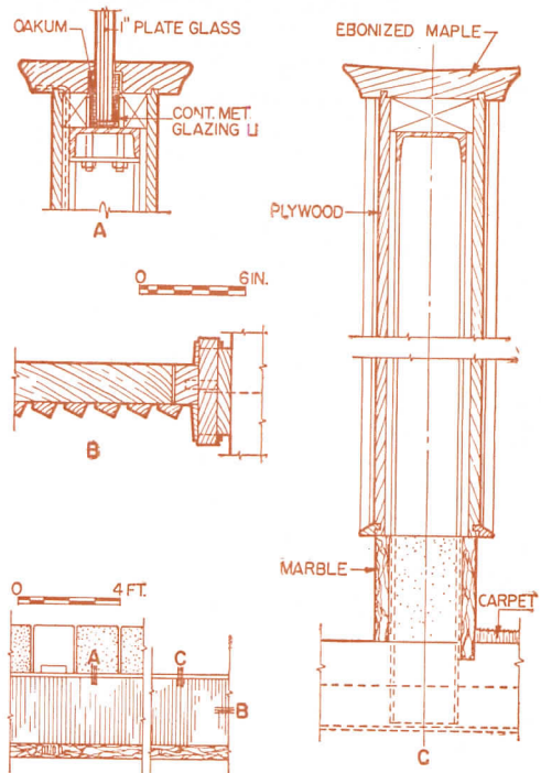
DETAILS- WOOD-PANELLED BANKING COUNTER
