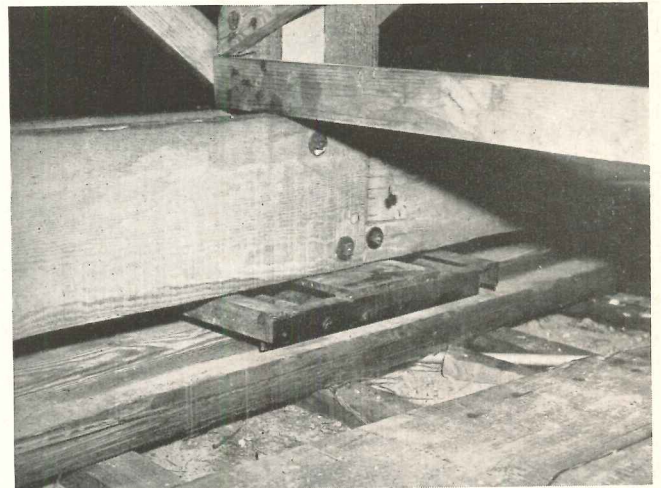
After the first 31-ft section was poured, forms were slid on dollies to the opposite side and finally to the middle section
