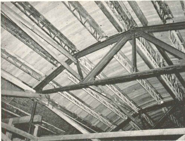
Five forms like this were used for pouring the 93-ft shells in three sections. Forms were built well because of future need
