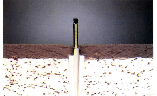
SPECTRA'S narrow \frac{3}{16} " exposed face, cut by a \frac{3}{16} " regress, offers 60% less visible metal at the ceiling plane for a refined look. Shown above with standard square-edge lay-in panels.
