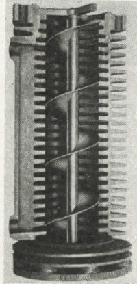
Cutaway of temperature control unit shows cooling fins, helicoid flighting
