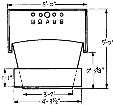
Fig. 2. Plan of organ console. The average organ console is about 4 ft. 3 in. high. An organ having more than three manuals requires 3 in. additional height for each manual added
