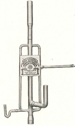
Prefab vent stack cuts construction time and saves up to 2 in. of wall thickness
