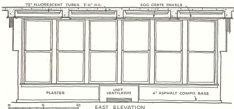
EAST ELEVATION
