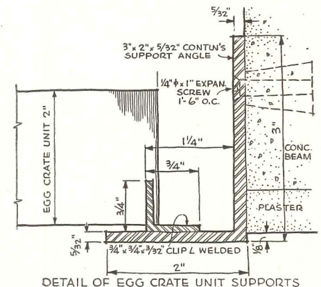
DETAIL OF EGG CRATE UNIT SUPPORTS
