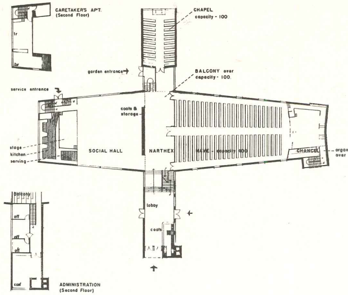
UPPER FLOOR
