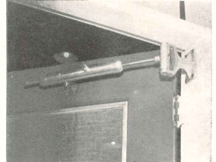
Door closer uses brake lining principle
