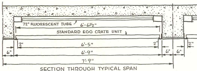
SECTION THROUGH TYPICAL SPAN
