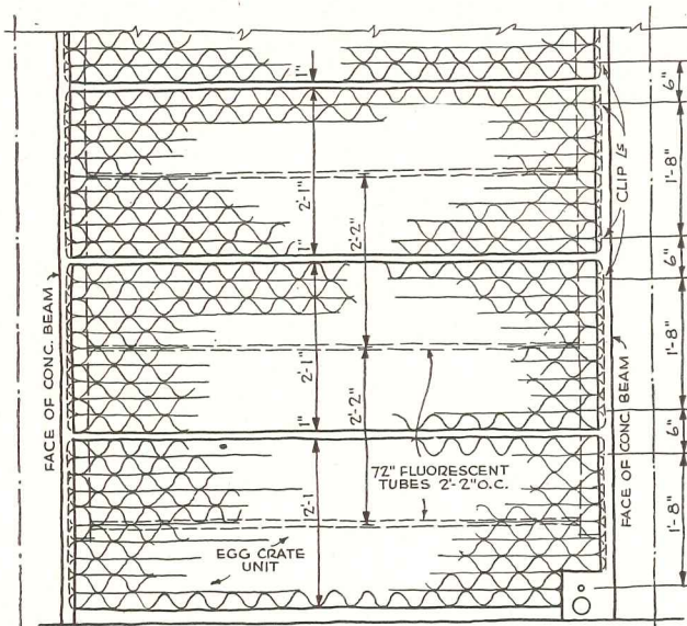
STANDARD EGG CRATE LIGHTING PANEL
