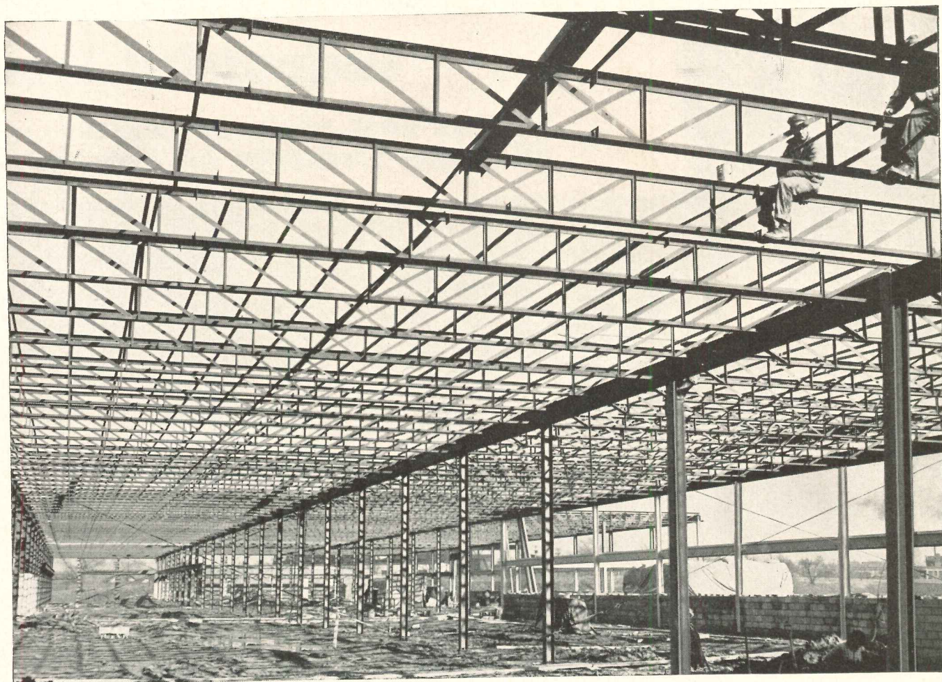
Bethlehem Longspan Joists in S. K. Wellman factory, Bedford, Ohio. Architect: Charles Bacon Rowley and Associates, Inc., Cleveland. Contractor: A. M. Hingley Company, Cleveland.
