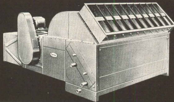
The Carrier Zoning Weathermaker, available in 5 sizes with cooling coils in 4 or 6 row direct expansion . . . or 4, 6 and 8 row cooling coils for brine or chilled water. Cooling capacities from 15 to 80 tons, 4100 to 16,400 cfm.
