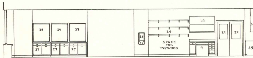
SECTION H-H
