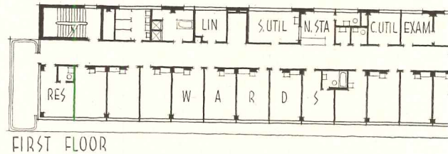
Tuberculosis Hospital also uses the long in-line scheme for nursing units, but has large rear extension for its laboratory and surgical facilities, as these procedures are largely special to a tuberculosis hospital
