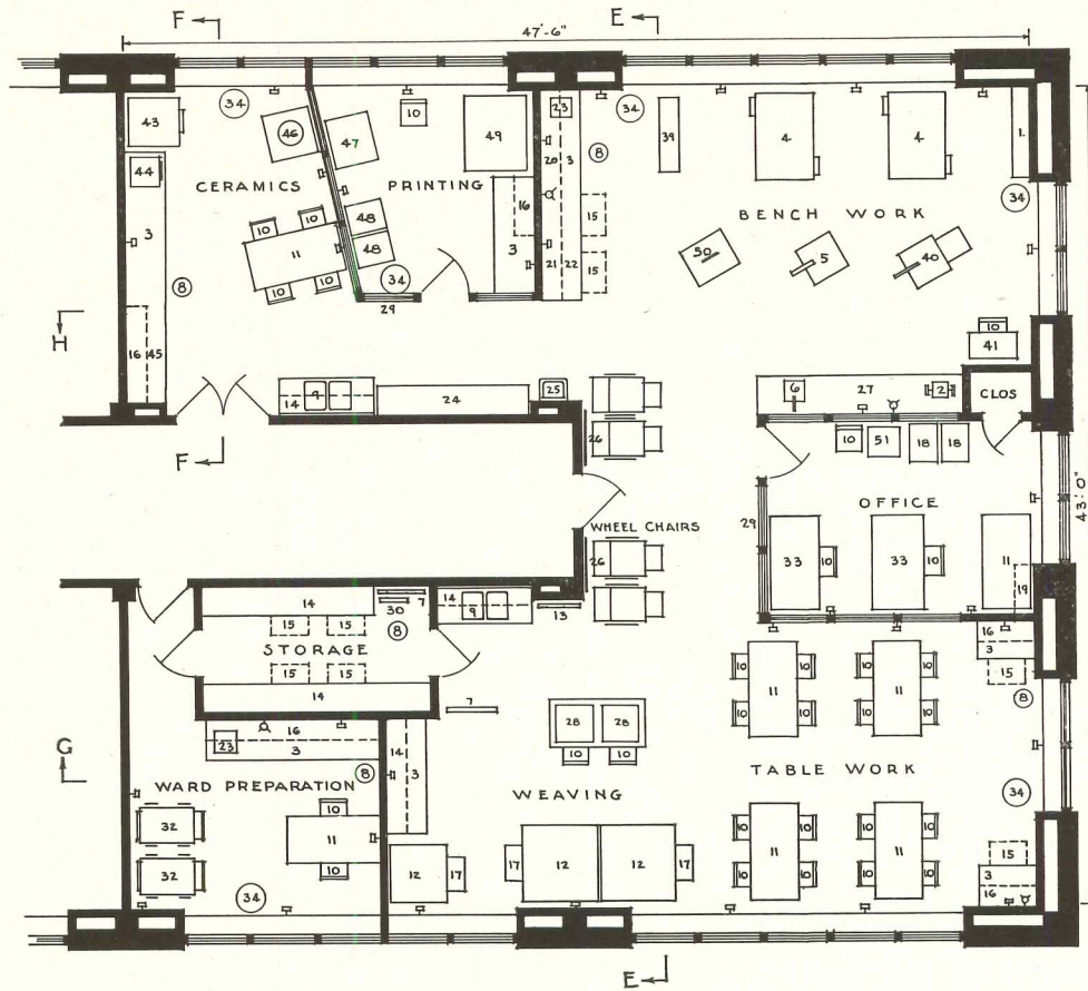
Plan for psychiatric, physical disability and general hospitals
