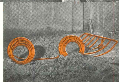
Installing condenser grid in wet clay prior to pouring basement floor.
