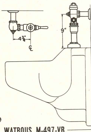
WATROUS M-497-VB Manually-operated exposed flush valve, top spud connection.
