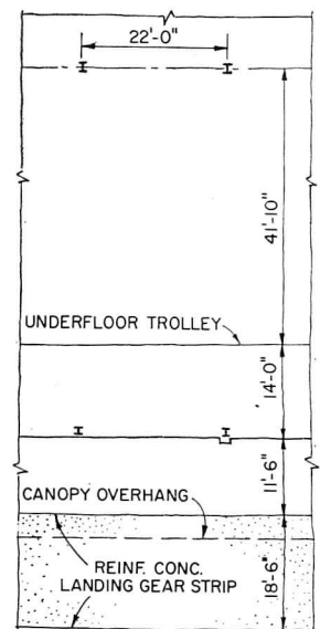
TYPICAL BAY
