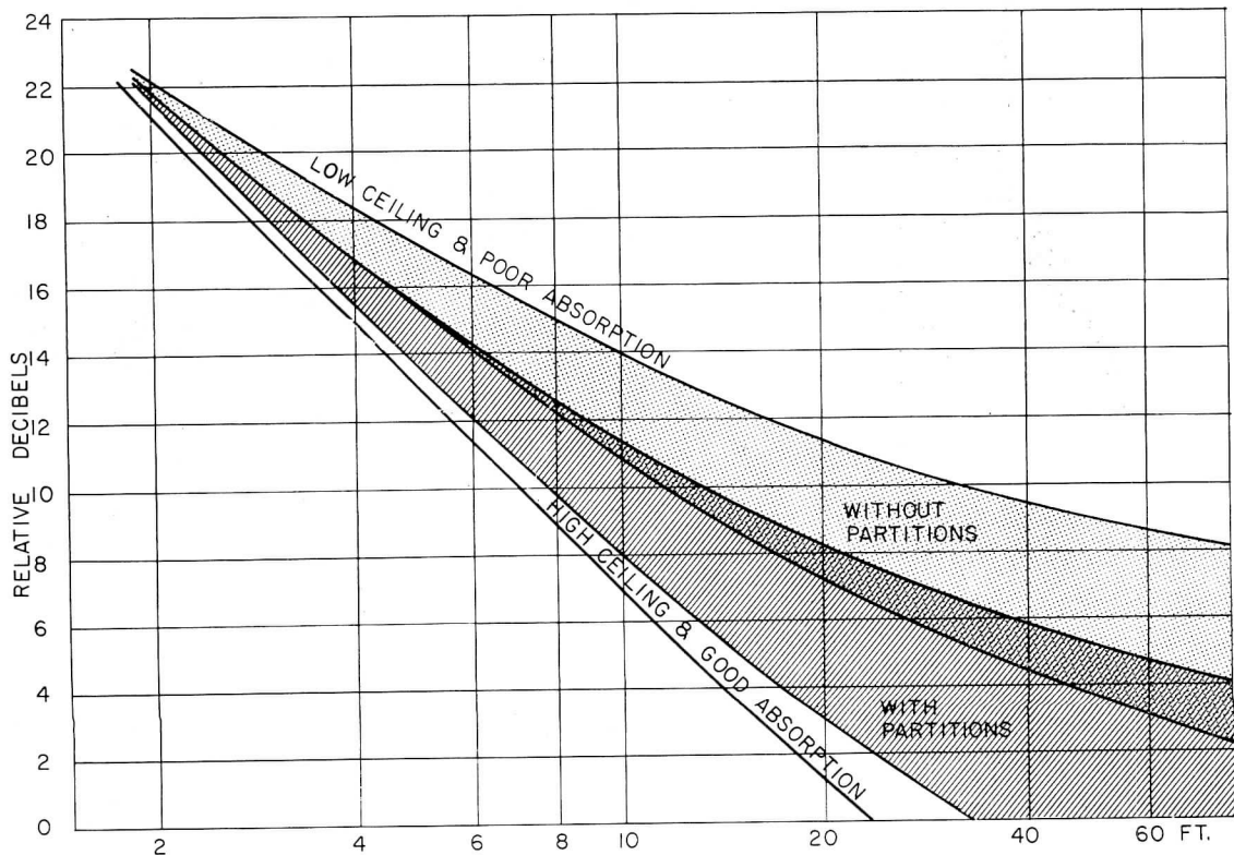
Fig. 6. How sound drops with distance in a large open office with different acoustical treatments. The upper shaded area is without office partitions; the lower shaded area is with 5-ft partitions
