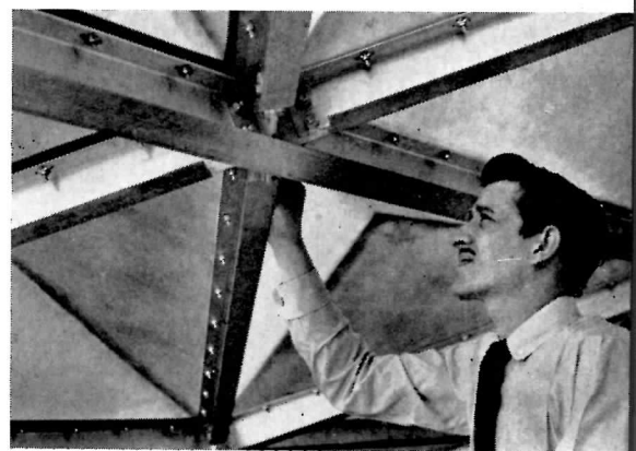
Plastic pans are attached to struts with anchor nuts. Connections between struts are by means of nuts and bolts
