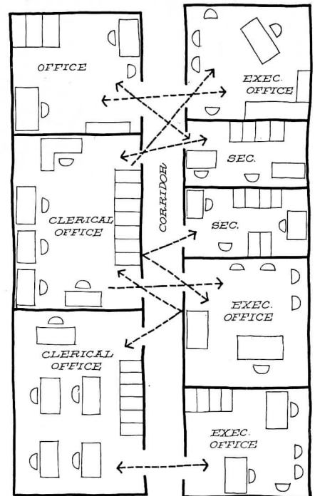
Fig. 2. A faulty arrangement of offices along a corridor. The presence of many doors at one point makes noise transmission likely, and it also causes traffic concentration in these areas
