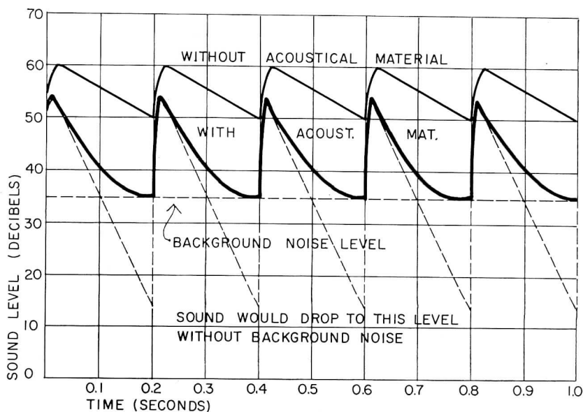
Fig. 5. A good acoustical ceiling reduces noise by causing sound to decay between impacts. Through the "picket fence" sounds can be heard more easily
