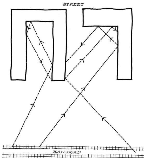
Fig. 1. An L- or U-shaped building may cause unforeseen focusing of sound around parts of the building
