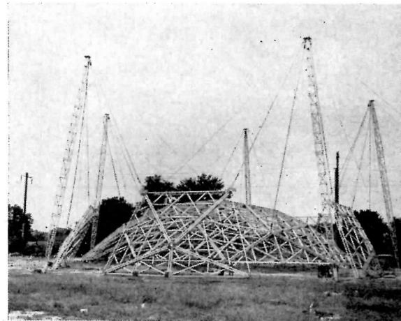
Final lift will sit the top assemblies on the ground assemblies, shown ready for moving under the sections when they are lifted
