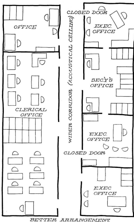
Fig. 3. The wider corridor covered with an acoustical ceiling isolates the office entrances. Two partitions have been eliminated. Executive offices are better isolated from the outside
