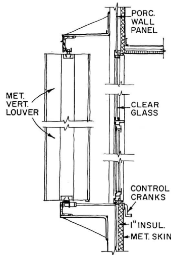
SECTION
