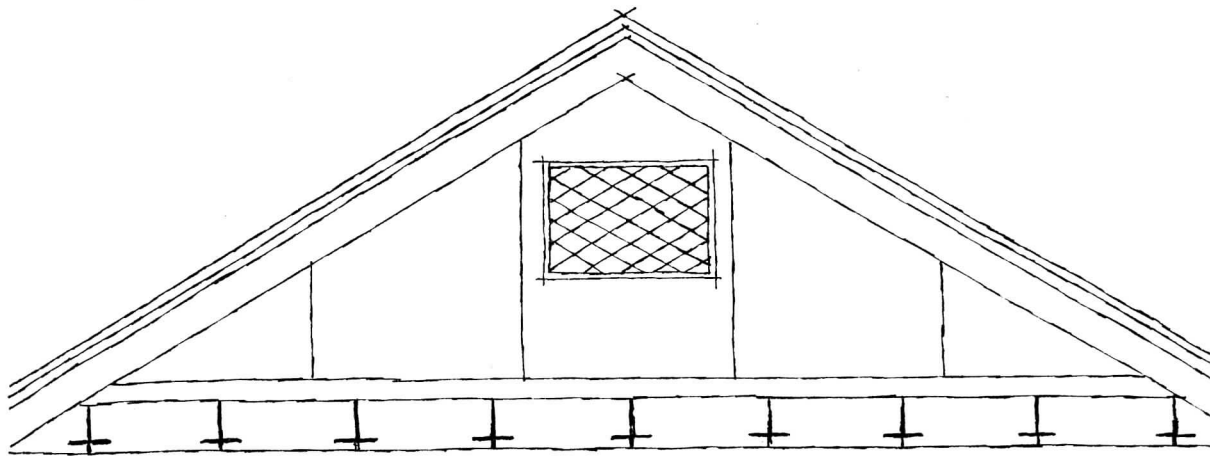
Fig. 2 With gabled roofs, it is important that at least one-half of the ventilated area between the suspended acoustical ceiling and the roof be in the upper portion of the air space.
