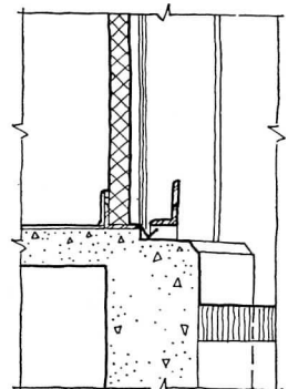
FLUTED WALL DETAILS
