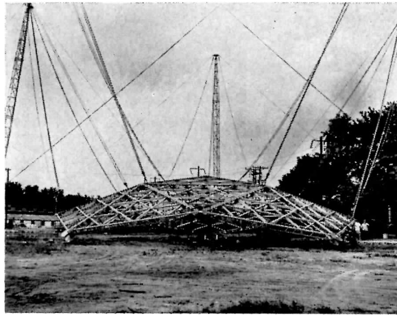
The top ring of five triangles and the second ring are lifted 3 ft off the ground with ginpoles to permit addition of next ring
