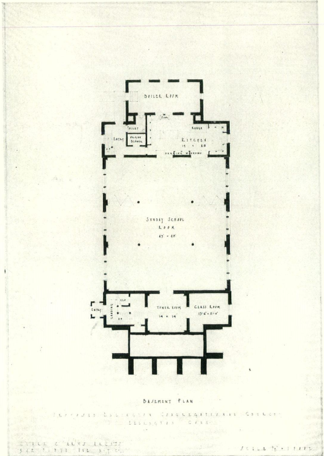
THE CONGREGATIONAL CHURCH, ELLINGTON, CONNECTICUT Clark and Arms, Architects
