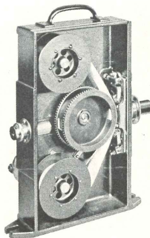
Interior View of the High-Speed Camera
