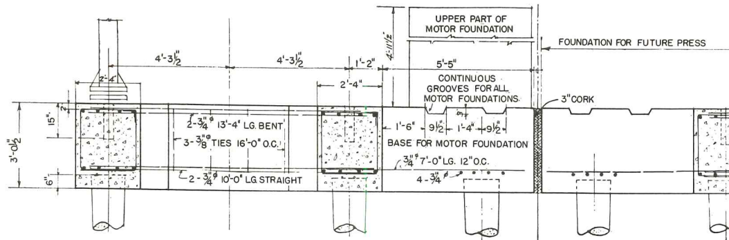
FIGURE 2 Section A-A
