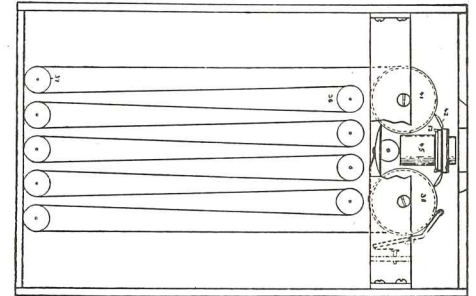
THE EDISON KINETOSCOPE PATENT DRAWING
