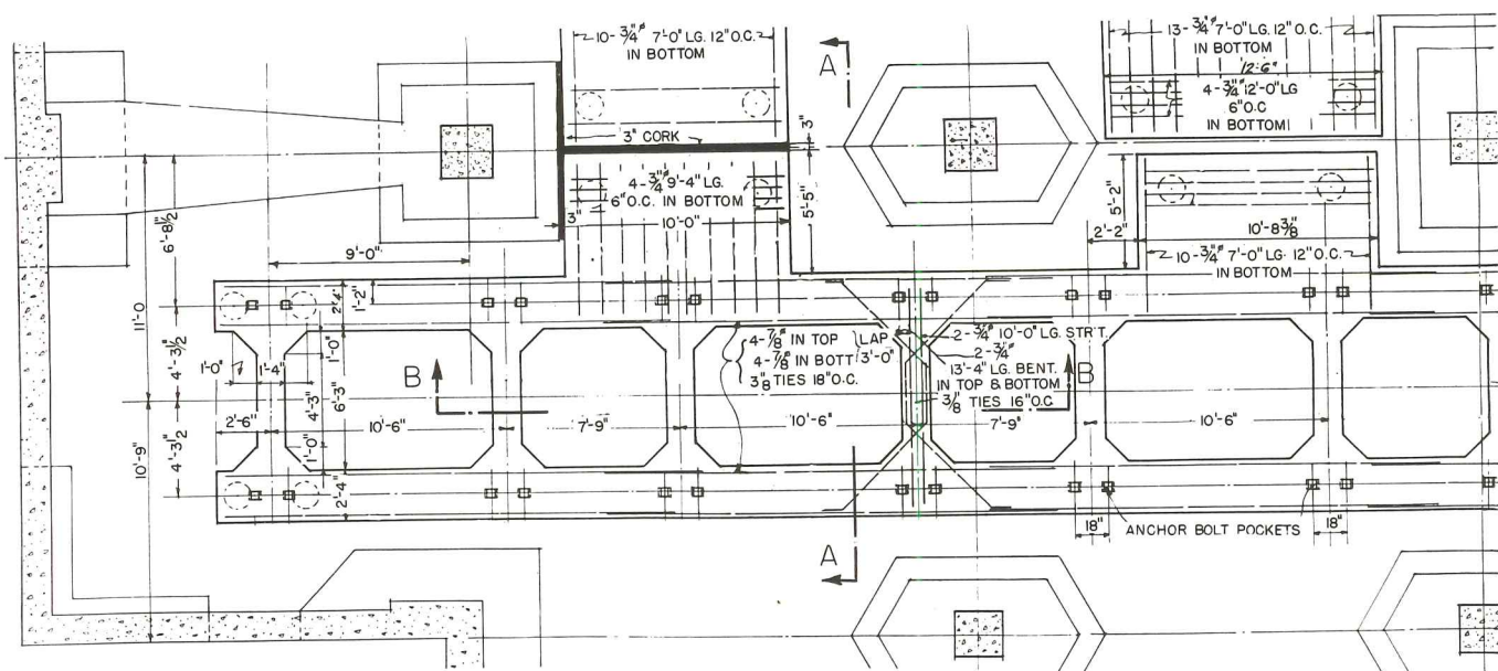
FIGURE 1 Plan of Press Foundation
