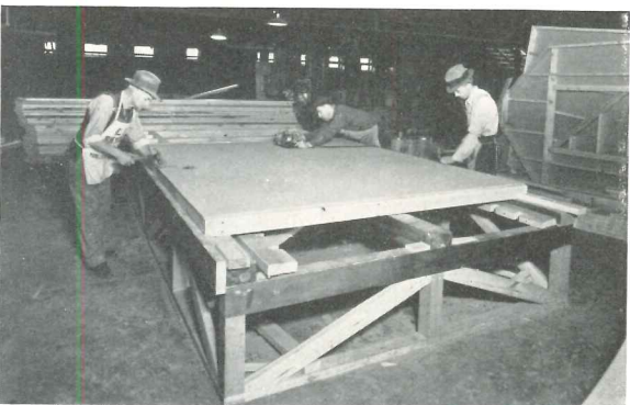
To both sides of units Homasote is fixed by means of special glue, special nails.
