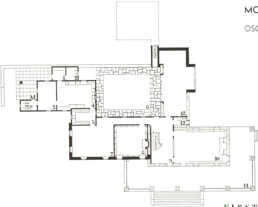
FIRST FLOOR PLAN SCALE 0 5 10 20
