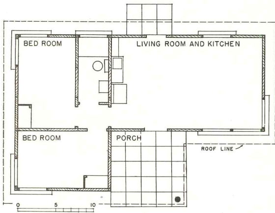
Floor plan
