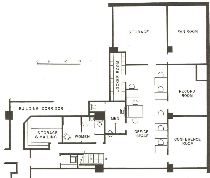
Basement plan
