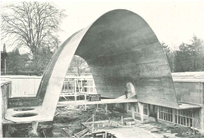
Hall, Zurich. Robert Maillart, Engineer. Vault is only about 3 1/2 in. thick.
