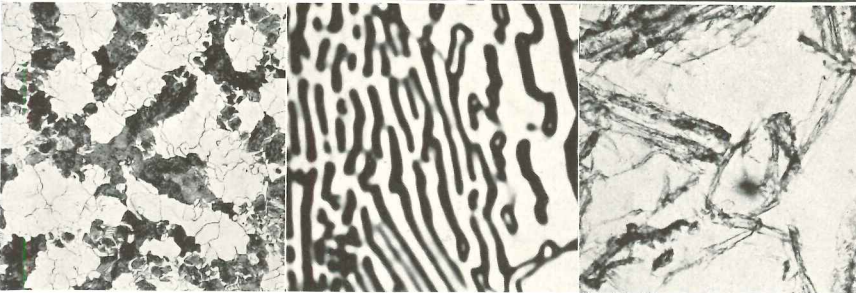
Researcher at metallographic microscope. Below, typical microphotographs (l. to r.): steel at 100 and 5,000 magnifications; filler for plastic, 175 magnifications.
