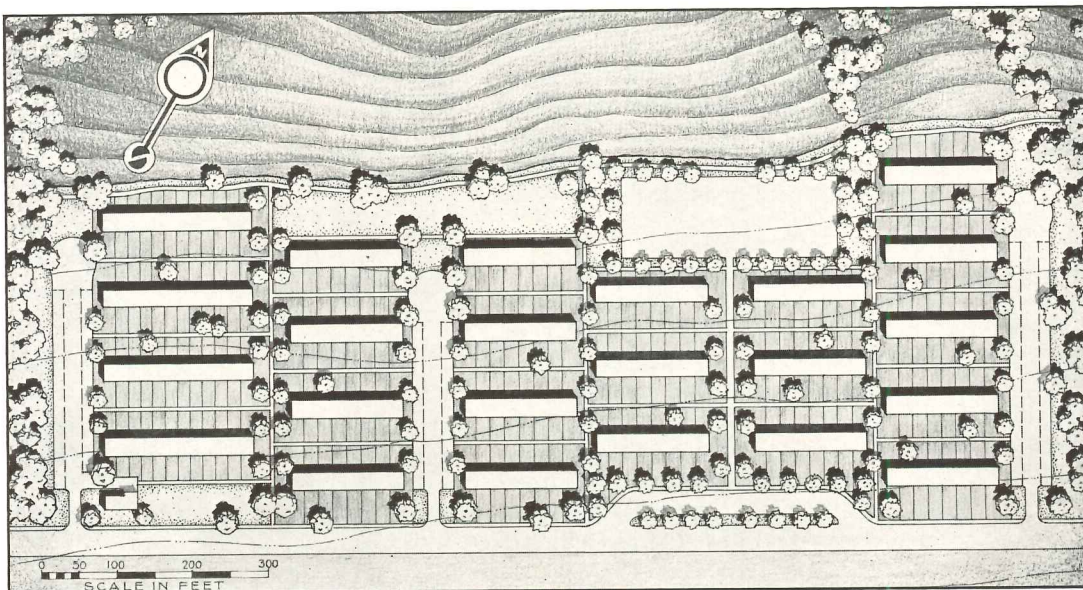
FIGURE 2: Sloping site with staggered arrangement of row-houses. Each dwelling unit has front and rear yard and end access for servicing. Curved de-sacs permit parking. Recreation areas on hillside above may be reached from every dwelling without traffic hazard, eliminating need for large common play lots. Building spacing is controlled primarily by orientation.
