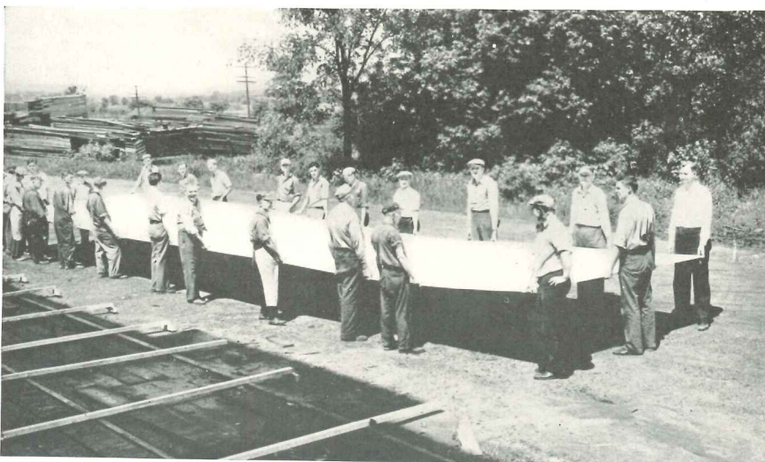
Greater control in fabrication makes possible resin-bonded plywoods. Ply-bond bus floor (above) is 9 x 46 ft., 5 plies thick, and weighs only 750 lbs.
