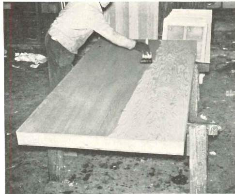
3. Panels are sized with Tung oil. Painting is done after house is assembled. . . .
