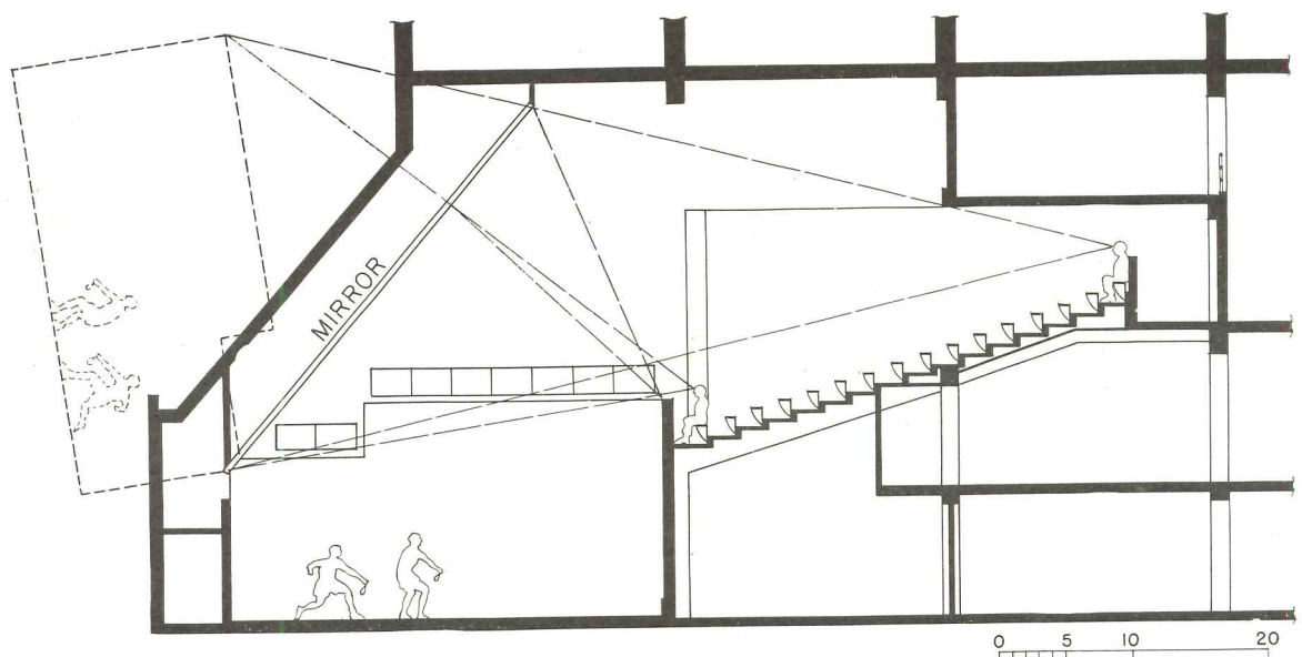
Section diagram
