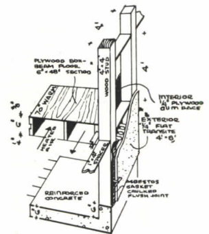
Construction detail
