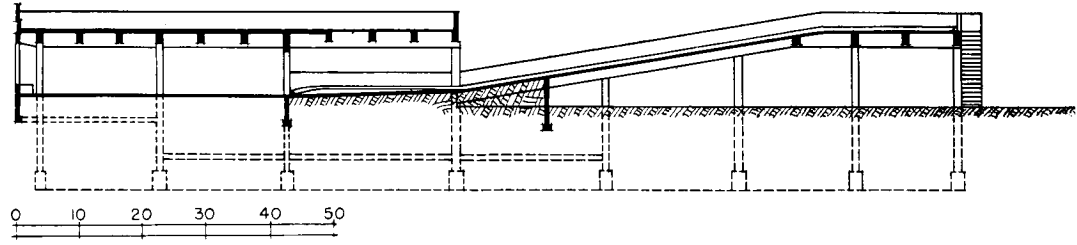
Section through ramp
