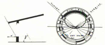
Summer solstice (about June 21); lat. 35°, long. 106°, at Santa Fe
