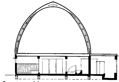
Section of barn
