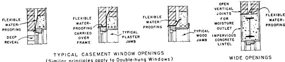
HEADS OF OPENINGS
