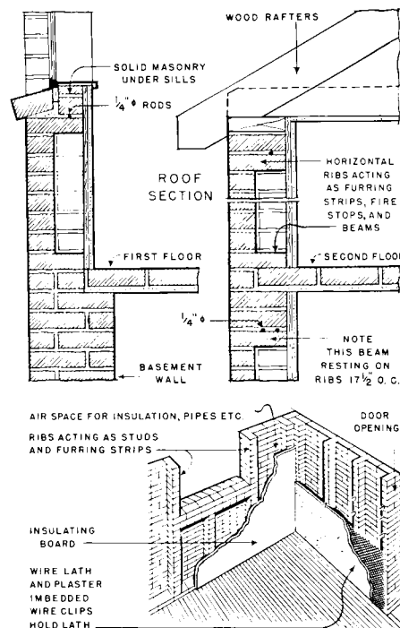
ECONOMY RIBBED WALLS
