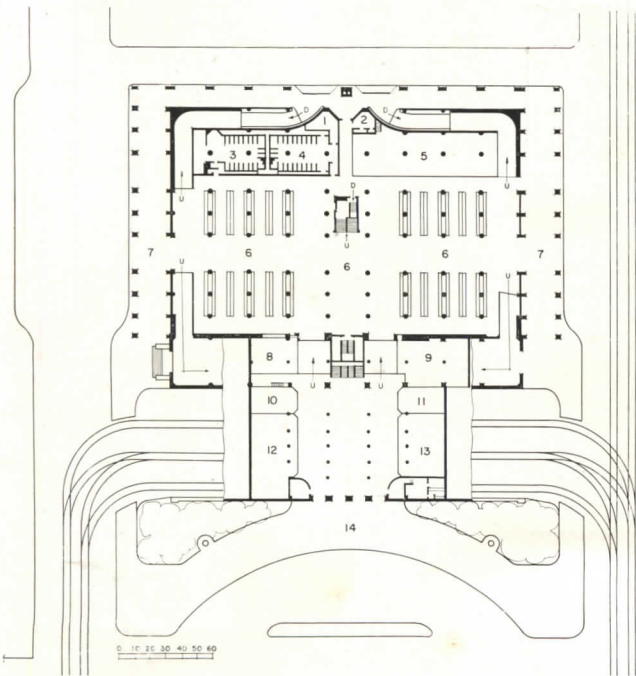
Ground floor: 1. Women's rest room. 2. First aid. 3. Men. 4. Women. 5. Restaurant, etc. 6. Waiting room. 7. Arcade. 8. Bakery. 9. Lunchroom. 10. Fruits. 11. Flowers. 12. Stand. 13. Stand.
