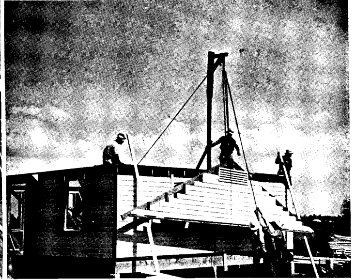
on precast concrete posts. Left, above, yard used for fabricating and storing wall and gable panels, roof trusses, etc.; right, hoisting complete gable-end. Panel sizes were limited to those which four men could handle (8 by 12 ft. typical).
