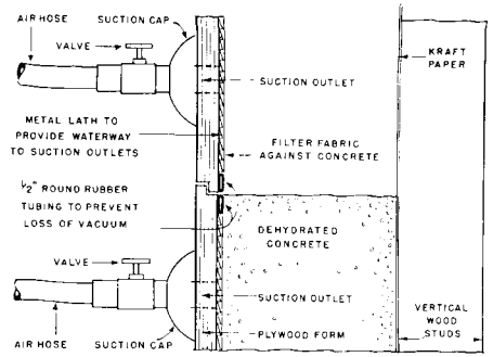
Form-work required for vacuum concrete: frame for paper backing is only form-support needed.
