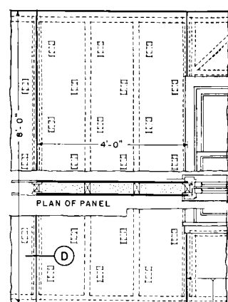
PANEL ELEVATION WINDOW UNIT
