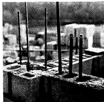
Making use of interstices in hollow block as pipe and conduit chases.
