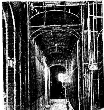
Metal lath and lath channels used in thin single or double partitions decrease both weight and space necessary.
