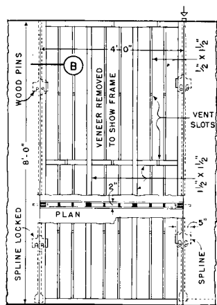
PANEL ELEVATION
