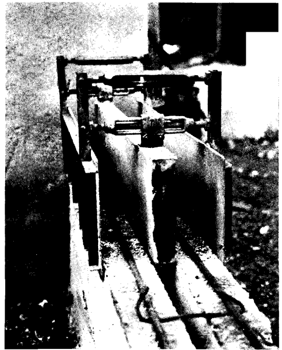
re-used quickly; successive layers are rapidly poured. Time and form costs are thus minimized. Forms come in sets, one unit for corners, one for straight walls, etc., and are supported by wall ties.
