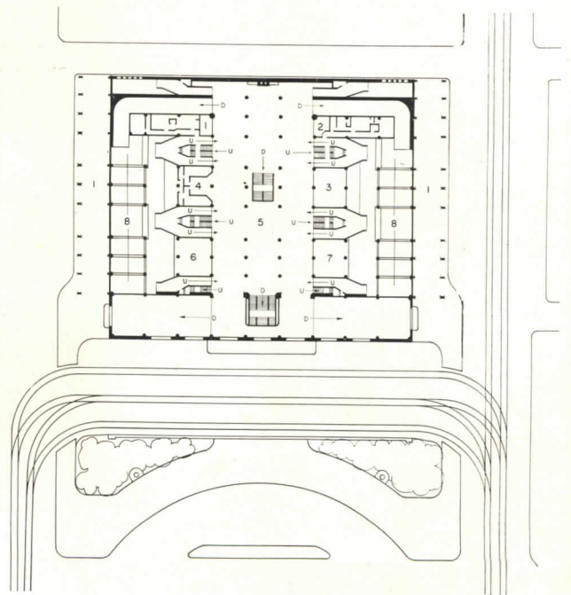
Mezzanine floor: 1. Travel agency and (or) ticket office. 2. Telegraph office. 3. Soda fountain and lunch counter. 4. Ticket office. 5. Concourse. 6. Drugstore. 7. Newsstand, candy. 8. Furred space.
