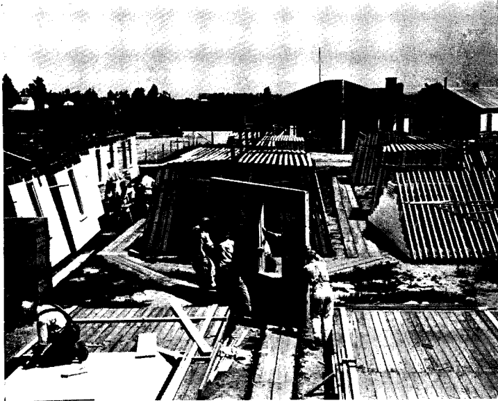
"Southeast Missouri Homes", constructed by the Farm Security Administration, were prefabricated in sections. Methods acceptable locally were used: panels have studs 2 ft. on centers; sheathing is omitted; floor framing is set
