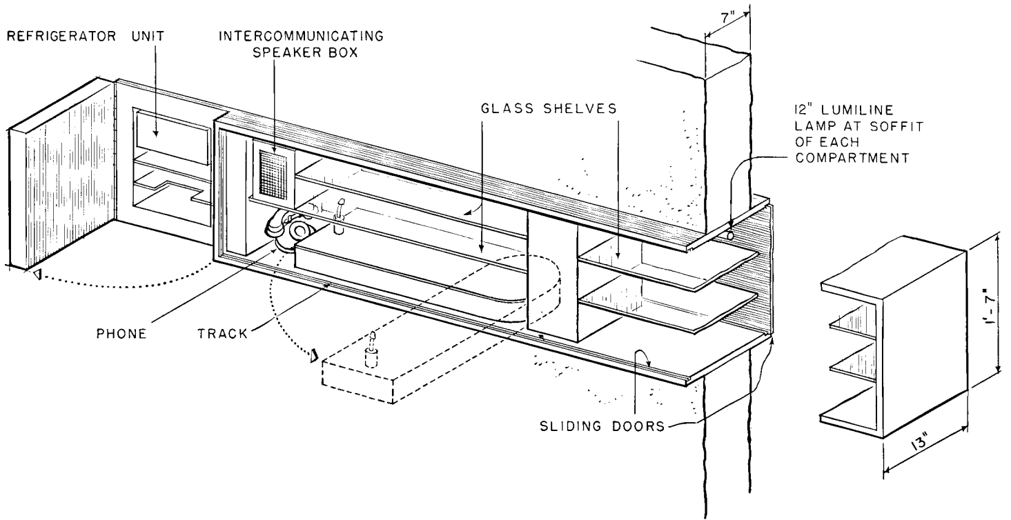
View of stainless-steel cabinet seen from treatment room No. 1, looking past the illuminated shelves into treatment room No. 2
