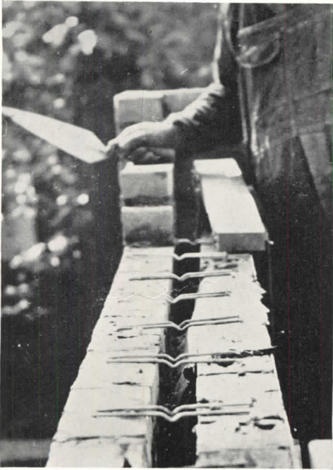
Method of laying cavity, or "barrier", brick walls: at left are shown metal wall ties crimped in the center to provide a drip for moisture; at right, chimney built according to "cavity" principle.
