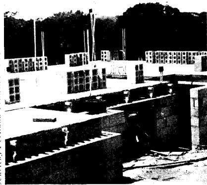
Concrete basement and first-floor construction provides a means of confining fires to the most common point of origin.
