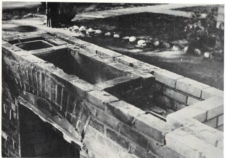
Method of laying cavity, or "barrier", brick walls: at left are shown metal wall ties crimped in the center to provide a drip for moisture; at right, chimney built according to "cavity" principle.
