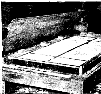
Prefabricated panels packed with loose mineral-wool insulation.
