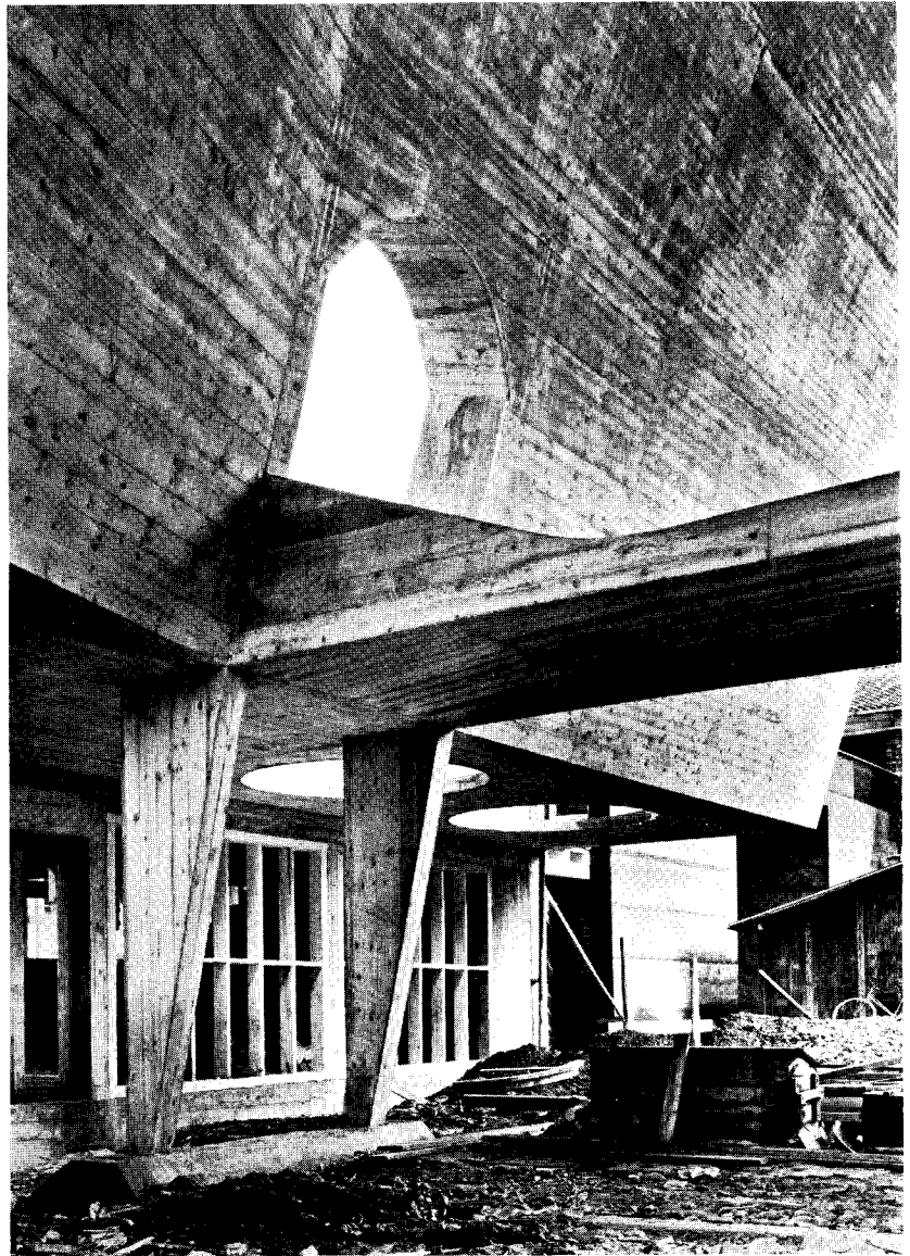
Four pillars, two on each side of the vault, are the only interior supports.
