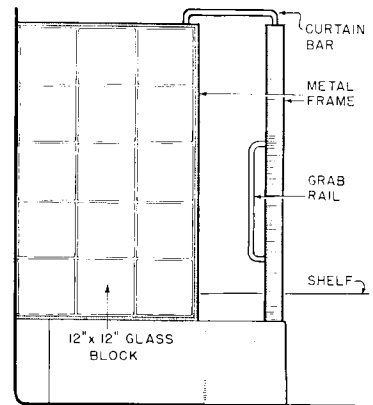
Glass-block partitions are used in the bathroom. Above is the corner tub, with side walls of glass block set in a metal frame, and a curtain bar provided over the opening.
