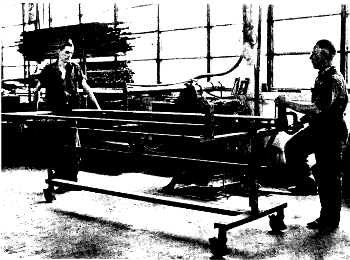
Hobart all-welded steel houses are completely shop-fabricated, trucked to the site, placed on the foundation, and hooked up to utilities. Walls and floors are thin, double-faced, reinforced steel, welded together and packed with insulation. Center, below, forming a door panel; and, bottom, houses on the production line.
