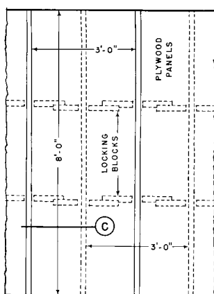
PANEL ELEVATION
