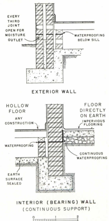
Adapted from "Principles of Modern Building"
