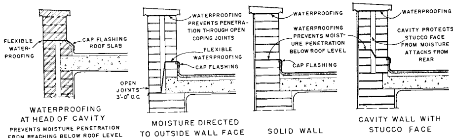
PARAPET CONSTRUCTION
