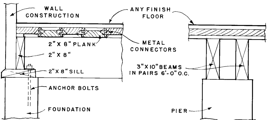
STAGGERED PLANKS SECTION PARALLEL TO GIRDER
