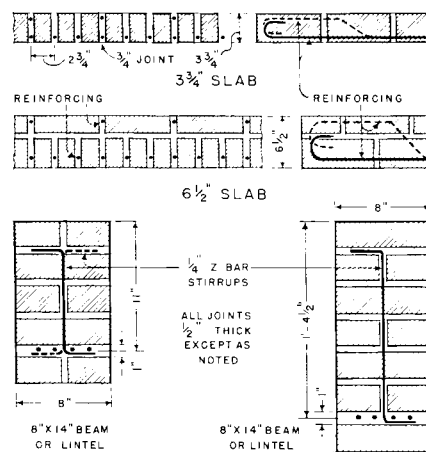
REINFORCED BRICK MASONRY
