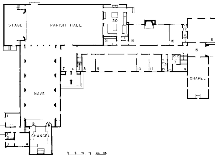
First floor: 1. Study. 2. Toilet. 3. Robe room. 4. Chair room. 5. Lectern. 6. Pulpit. 7. Northex. 8, 10, 11. Classrooms. 9. Primary Room. 12. Wash room. 13. Toilet. 14. Stairs. 15. Lobby. 16. Beginners' Room. 17. Toilet. 18. Nursery. 19. Ladies' Parlor. 20. Kitchen. 21. Pantry.
