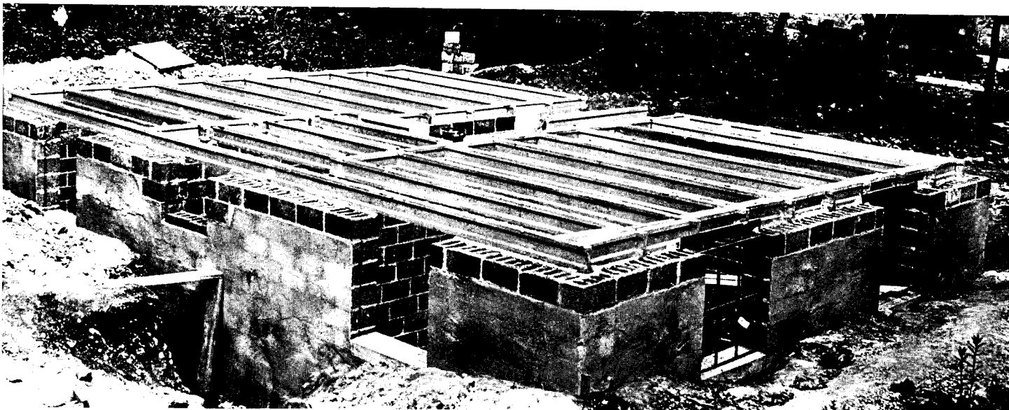
Typical concrete construction: block foundations with parge-coat waterproofing, precast joist floor ready for pouring the slab.
