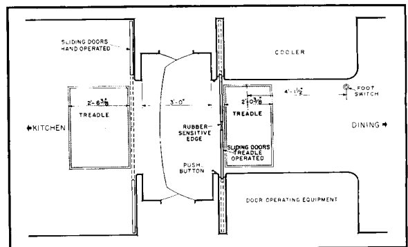
Diagrammatic plan, showing location of important elements.
