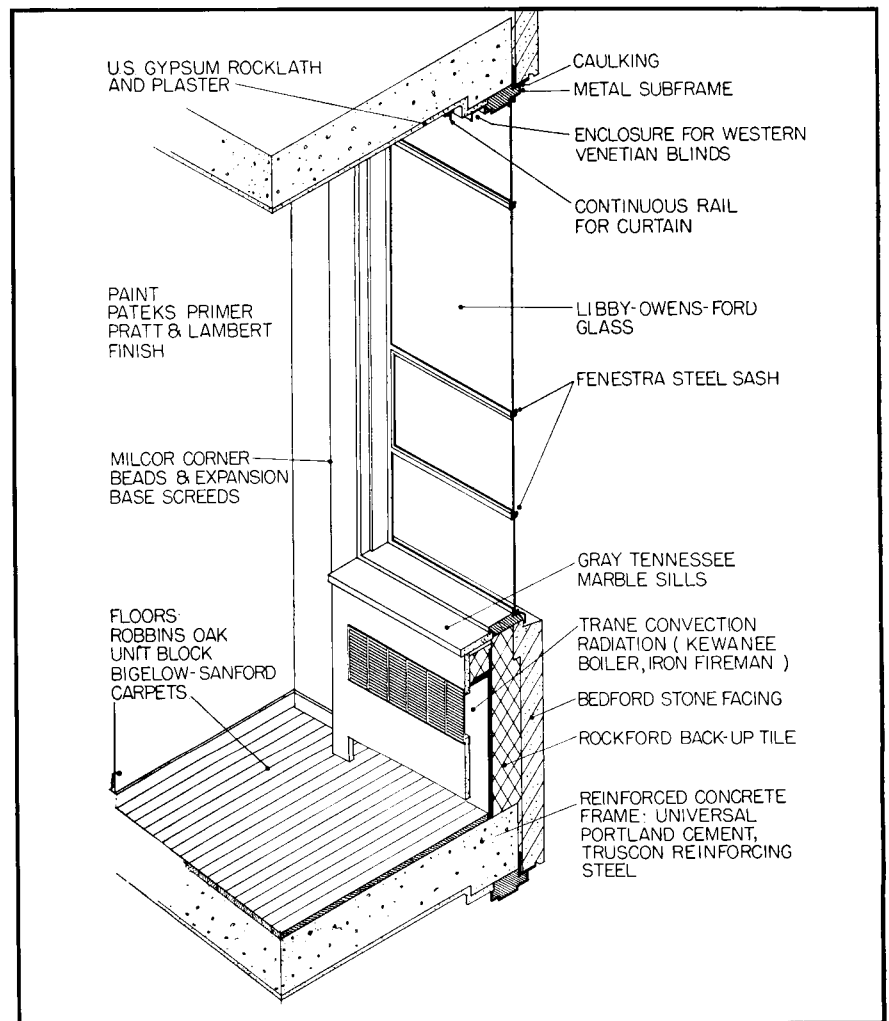
Construction, typical bay
