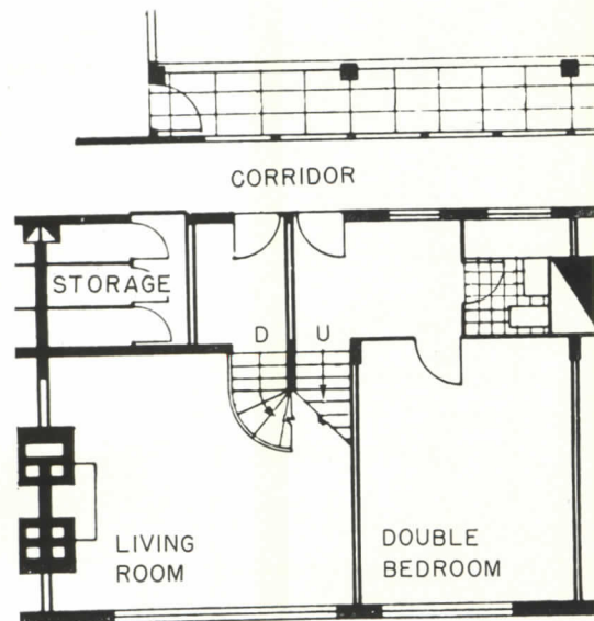
MIDDLE LEVEL, typical "three-two" unit.
