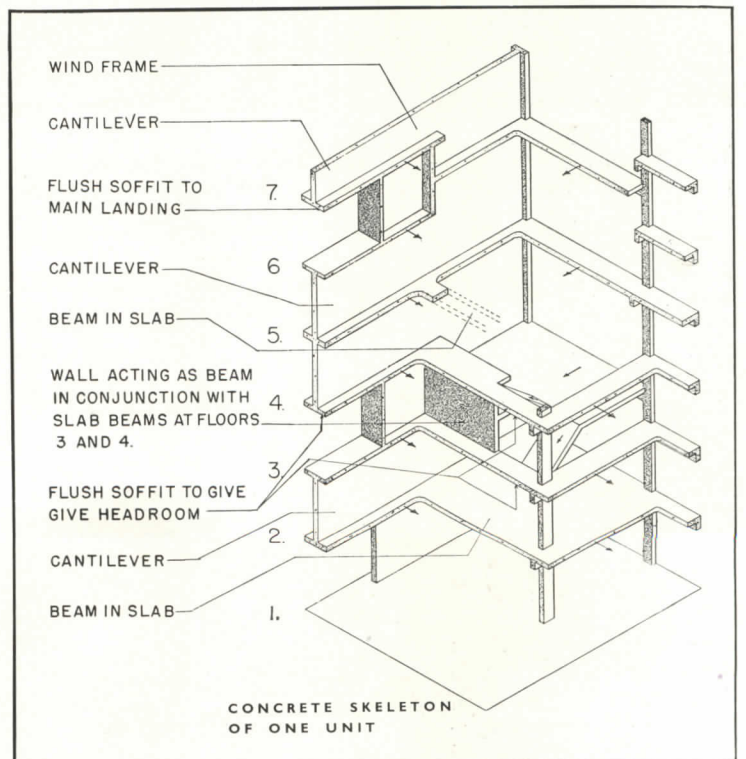
Continuous concrete frame frees interior space.
