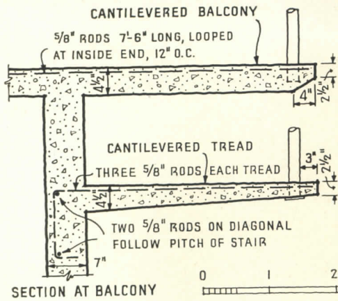
Detail of cantilevered balcony and stair leading from terrace. Uprights of the balustrade are of 1½-in. pipe, which have been drilled to support wood rail dowels.
