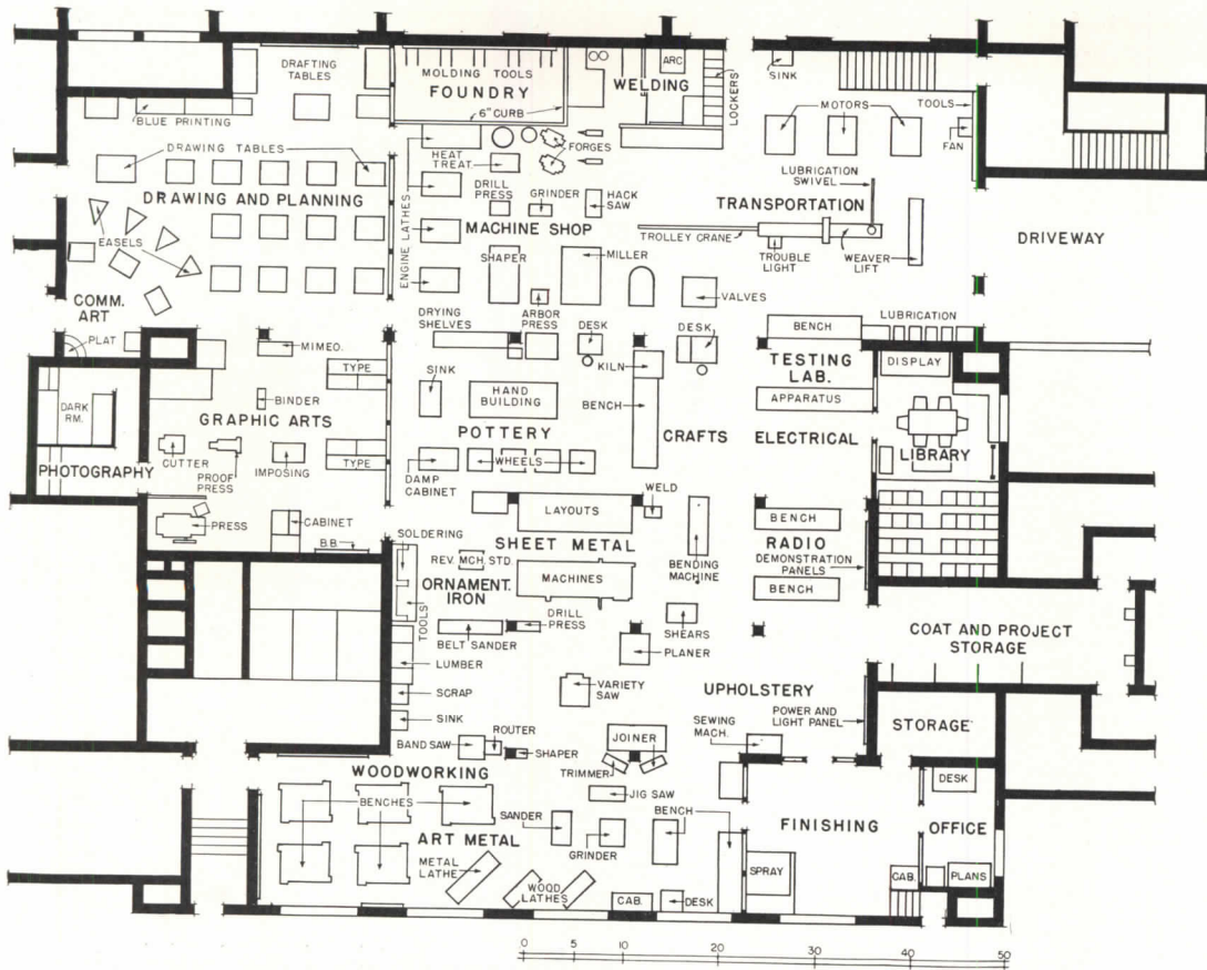
"Arts and Industries" laboratory in Cambridge, Ohio, High School; E. W. Austin, Architect; Wm. E. Warner, Educational Consultant. Note interrelation of such areas as transportation (automotive), machine shop and foundry, metals and woodworking, etc. Dust and noise are eliminated from library, finishing room, graphic arts and drawing rooms by soundproof steel and glass partitions.
