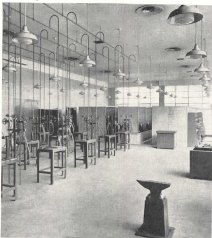
Overhead services, welding shop, South Vocational High School.
