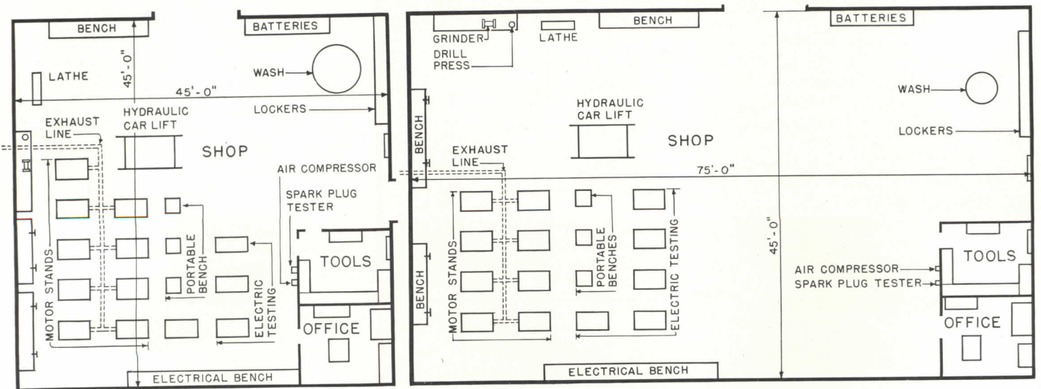
Machine shops for (left) 10-15 students, (right) 15-25 students, indicating relationship of equipment and space allocations for tool room and instructor's office.
