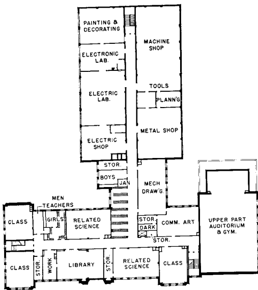
Second floor contains shops for which grade-entrances were not essential. There is a glass-enclosed planning room centrally located in each group of shops.
