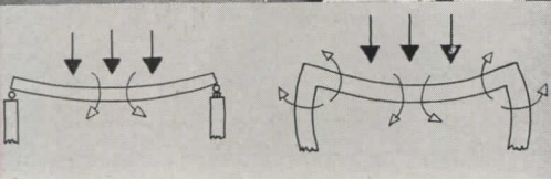
Fig. 8: Whether the connection be hinged (left) or rigid (right), steel as a material is well-adapted to either, with a practical monopoly on the former.
