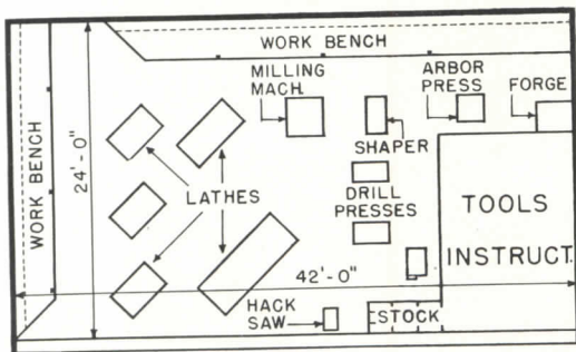
Machine shops for (left) 10-15 students, (right) 15-25 students, indicating relationship of equipment and space allocations for tool room and instructor's office.
