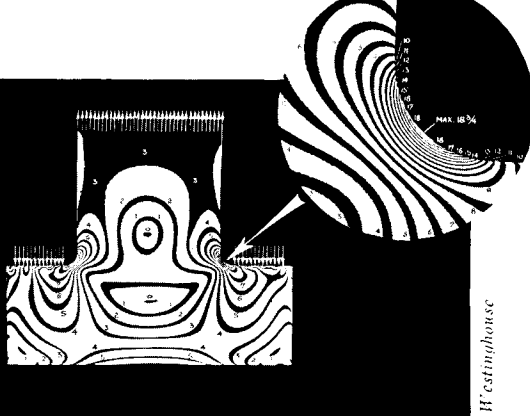
Fig. 4: Of great importance to the building field are current studies in photoelasticity. By means of them, our theories of structure are being checked, refined, and greatly extended.
