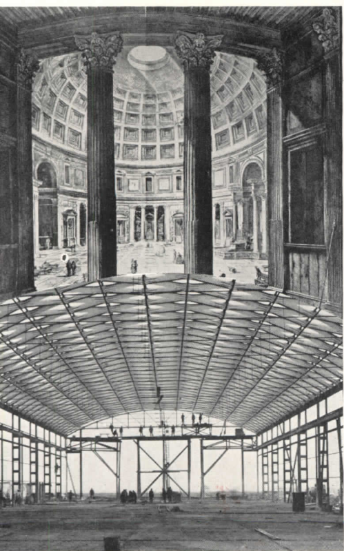
Fig. 3: The material at hand largely determines the specific structural form. Thus, concrete (top) and steel (bottom) were equally adapted to great spans.
