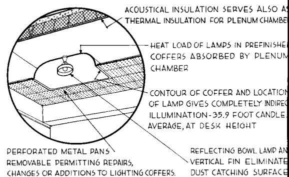
Light-coffer detail
