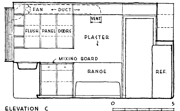
ELEVATION C
