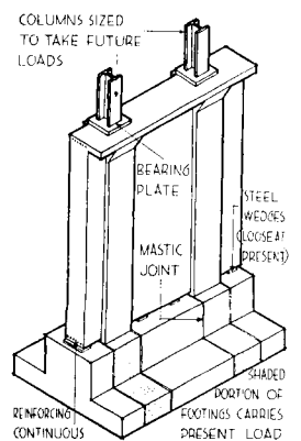
Detail of footing
