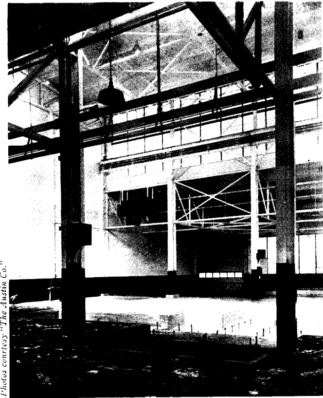
Above and at left, three interiors of a 34,000-sq.-ft. addition to the Cleveland Punch and Shear Works, Austin-designed, of which the frame is entirely welded. Note provisions for heavy machine installations. Crane aisle spans 55 ft.; low side aisles, 50 ft. At right, interior of a "windowless" plant, also Austin-designed, where complete control of atmosphere aids precise manufacturing.
