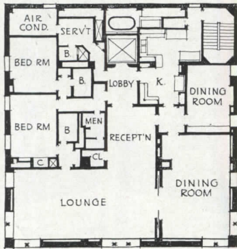
30 TH FLOOR
