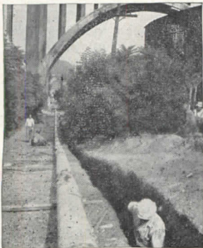
Welded into a single piece 700 feet long, this pipe was lowered into the shallow trench beside it, a section of the 2000 foot connection to the city main.
