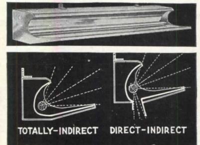
Reflector unit for germicidal lamp
