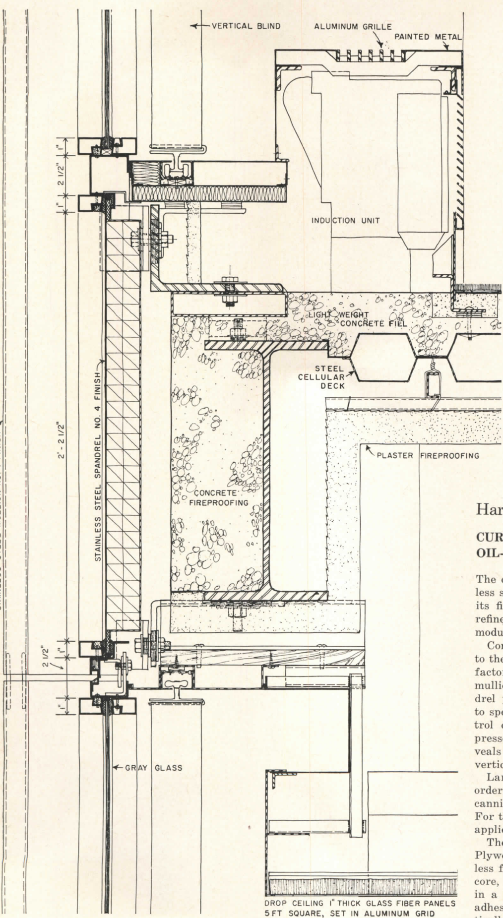
DETAIL A-A VERTICAL SECTION THROUGH SPANDREL
