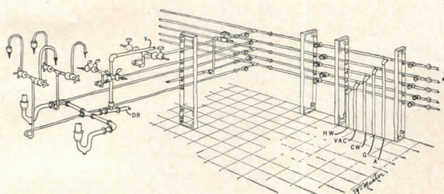
Figure 1. Laboratory Piping Diagram
