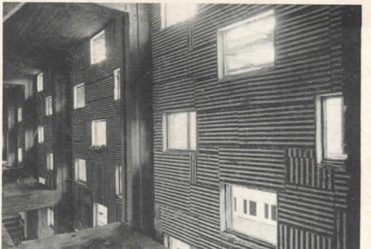
Figure 4. Polystyrene foam on the walls of a swimming pool hall supports the plaster and provides thermal and condensation insulation
