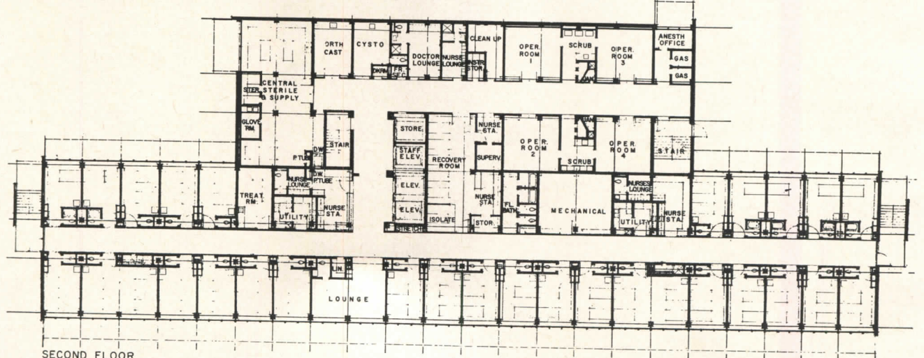
SECOND FLOOR
