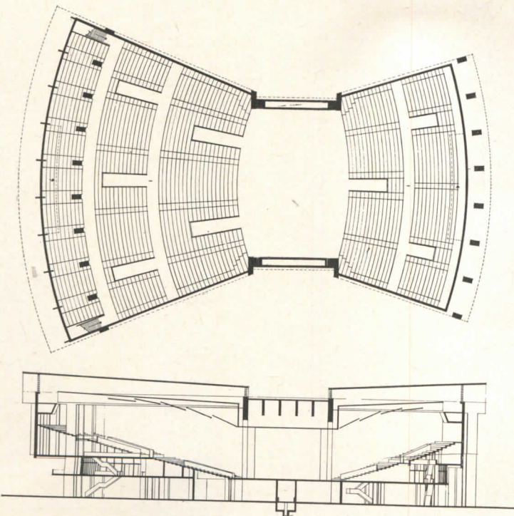
Auditorium plan and section. It has been designed to accommodate the large number of people required for special occasions, but it can also be divided into smaller auditoriums for lectures, music performances, etc. The two smaller auditoriums, seating 3,220 and 1,150, face each other across a central flat stage area which can be partitioned off in a number of different ways. When in use as a single large space, an additional 650 seats may be placed on the central stage providing a total seating capacity of 5,020
