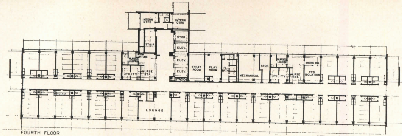
FOURTH FLOOR
