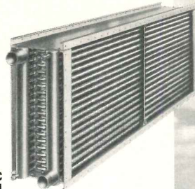
Type C chilled water coil
