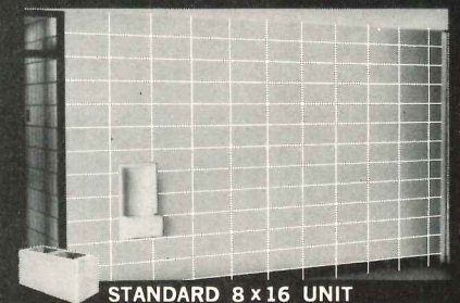
STANDARD 8 x 16 UNIT
