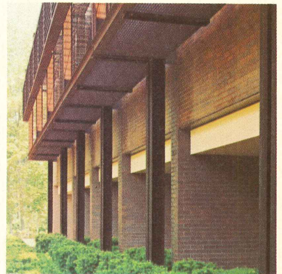
Shrubbed beds of crushed stone serve as drains to catch the oxidized run-off from the maturing Weathering Steel.
