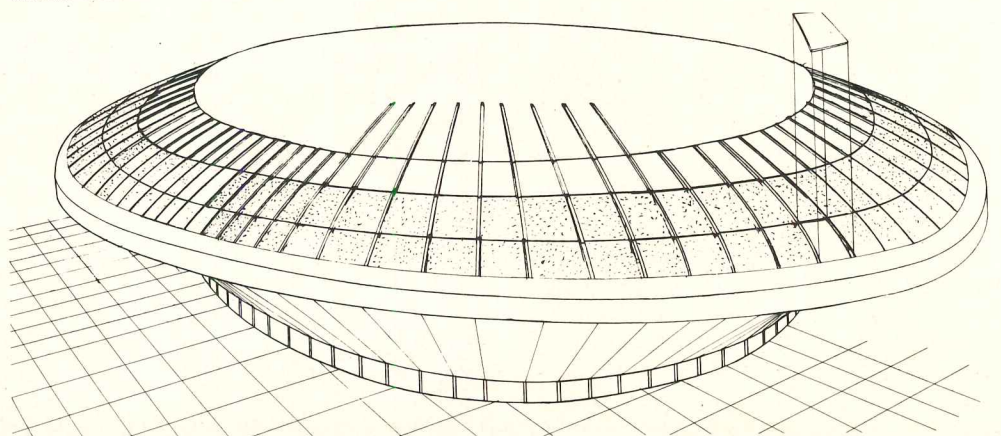
This proposed design utilizes precast concrete elements for the "cone" section and cantilevered portion of the roof. Center of roof is an inflated stainless steel "pillow." Model of similar structure is above.
