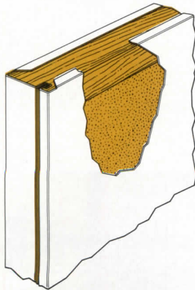
Vinyl thermal break locks steel skins together while separating exterior and interior surfaces to inhibit temperature penetration and condensation.
