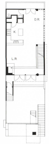
SECOND FLOOR
