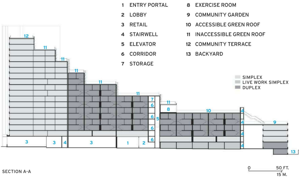
THE GREEN WAY The planted roofs of Via Verde—many of which are accessible to residents—spiral down from a 20-story tower, meeting the ground with an amphitheater-like set of steps. On the terraced roofs grow an evergreen grove, an apple orchard, and vegetable plots.
