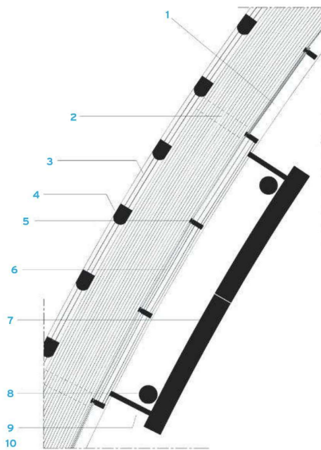
FACADE DETAIL
