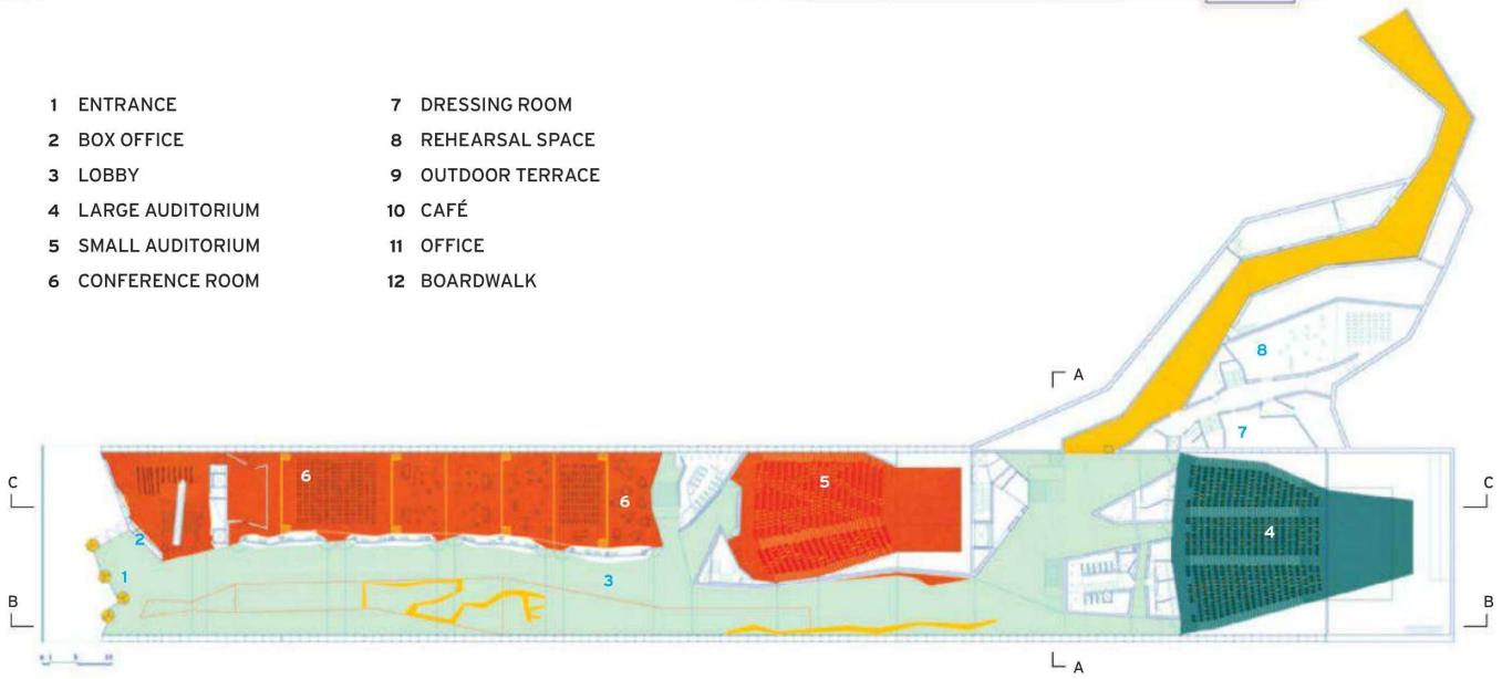
GROUND LEVEL PLAN
